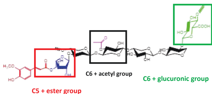
Figure 1. Representation of a hemicellulosic fragment, a glucuronoarabinoxylan composed of a D-xylose unit ( \beta -1-4 equatorial position), \alpha -1,3-L-arabinose with ferulic acid, acetyl and glucuronic acid groups. 10
