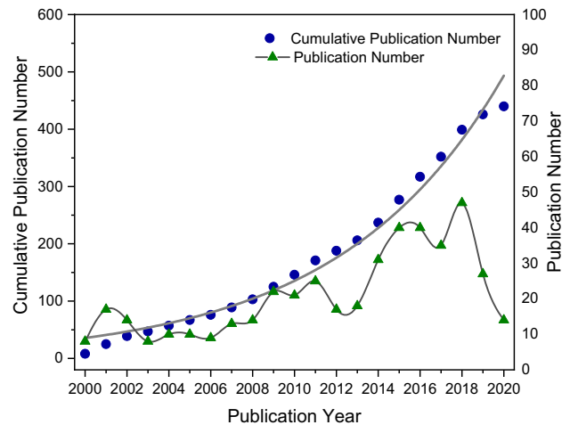
Fig. 1 Publications of WTS studies in the last 20 years based on Web of Science search
