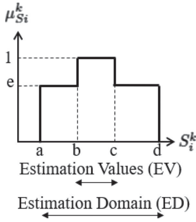
Figure 1. Possibility distribution \mu_{S_i}^k(S_i^k) of a criterion k for a solution S_i .
