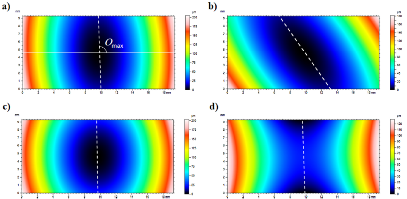
Fig. 4. 3D polynomial distortion determined on the top surface of conventional bridge specimens built with P = 300 \text{ W} and v = 1800 \text{ mm}\cdot\text{s}^{-1} and various strategies: (a) unidirectional zigzag scanning with \theta = 0^\circ or (b) \theta = 45^\circ , (c) inwardly or (d) outwardly concentric scanning [the white dotted line indicates the O_{\max} orientation corresponding to the bending axis].
