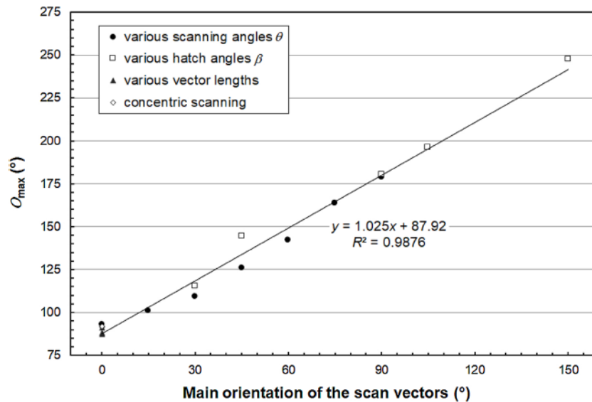
Fig. 11. Linear relationship between the orientation O_{\max} of the maximum curvature and the main orientation of the scan vectors, for all conventional bridge specimens built with the same process parameters ( P = 300 \text{ W} , v = 1800 \text{ mm.s}^{-1} ).
