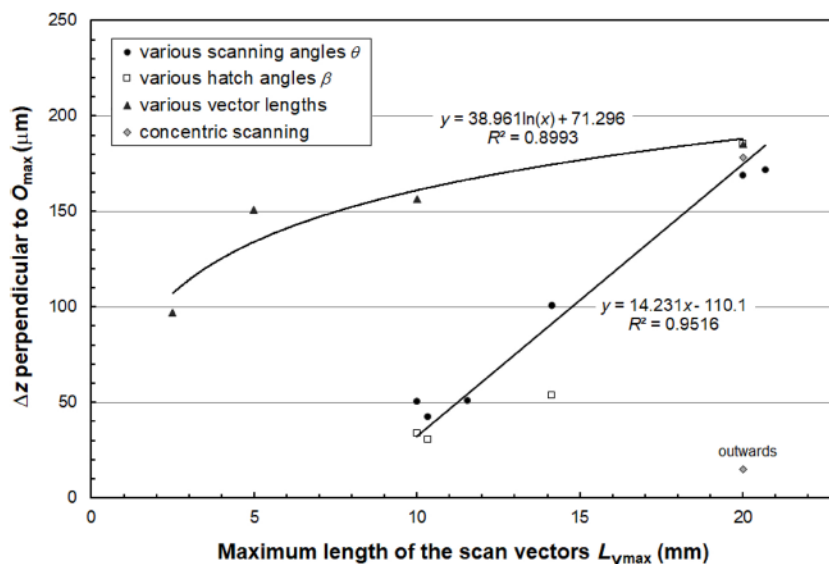
Fig. 15. Evolution of the distortion amplitude \Delta z measured perpendicular to O_{max} as a function of the maximum length of the scan vectors L_{vmax} , for conventional bridge specimens built with the same energy density ( E_v = 32.7 \text{ J} \cdot \text{mm}^{-3} ) and various scanning strategies.
