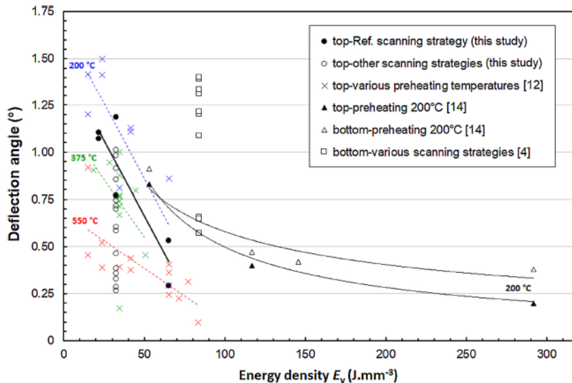
Fig. 14. Effect of the volumetric energy density E_v on the deflection angle (used to assess the distortion amplitude): experimental data from the present study and data found in literature works (Kruth et al [4], Malý et al [12], Mishurova et al [14]). The temperature indications refer to a preheating of the baseplate.
