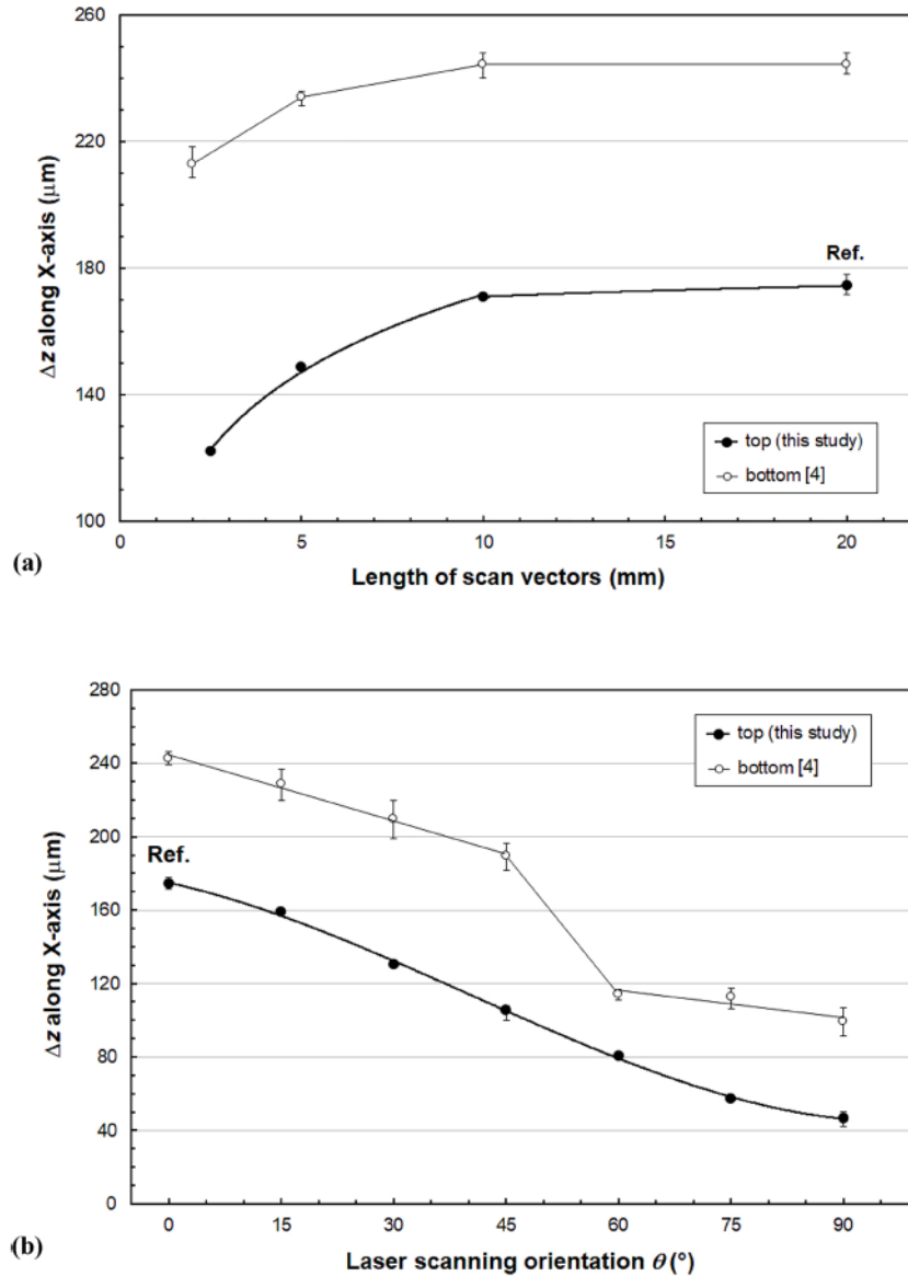
Fig. 8. Effect of (a) the scan vector length L_v and (b) laser scanning orientation \theta on the distortion amplitude \Delta z along x-axis of conventional bridge specimens built with a unidirectional back-and-forth scanning: comparison with the results of Kruth et al. [4].
