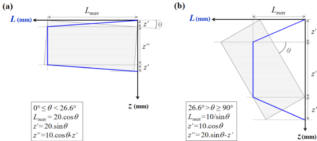
Fig. 3. Trigonometric approach to calculate the length of the scan vectors as a function of the laser orientation \theta on conventional bridge specimens: (a) for 0^\circ \leq \theta < 26.6^\circ ; (b) for 26.6^\circ < \theta \leq 90^\circ .
