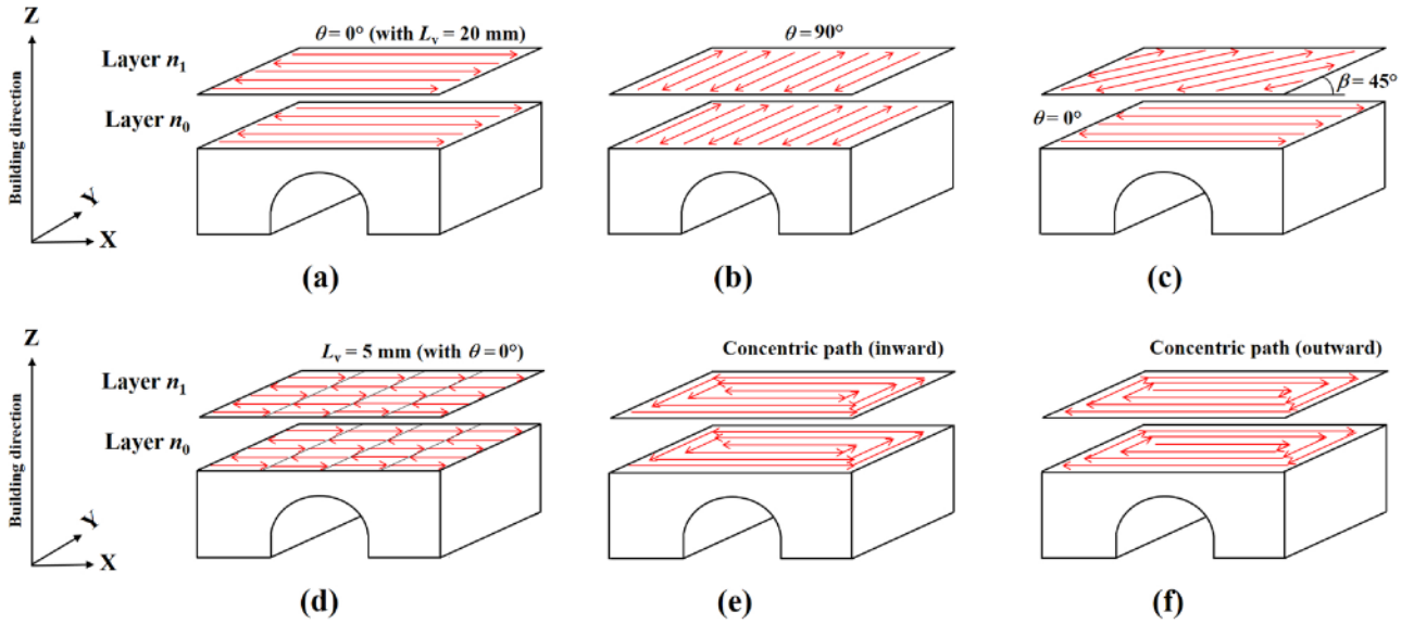
Fig. 2. Examples of investigated laser scanning strategies: unidirectional zigzag pattern with (a) \theta = 0^\circ (reference test) or (b) 90^\circ , (c) hatch rotation with \beta = 45^\circ , (d) scan vectors of length reduced to L_v = 5 mm; (e) inwardly and (f) outwardly concentric scanning. (The two layers shown were sequentially repeated until reaching the last layer n_L ).
