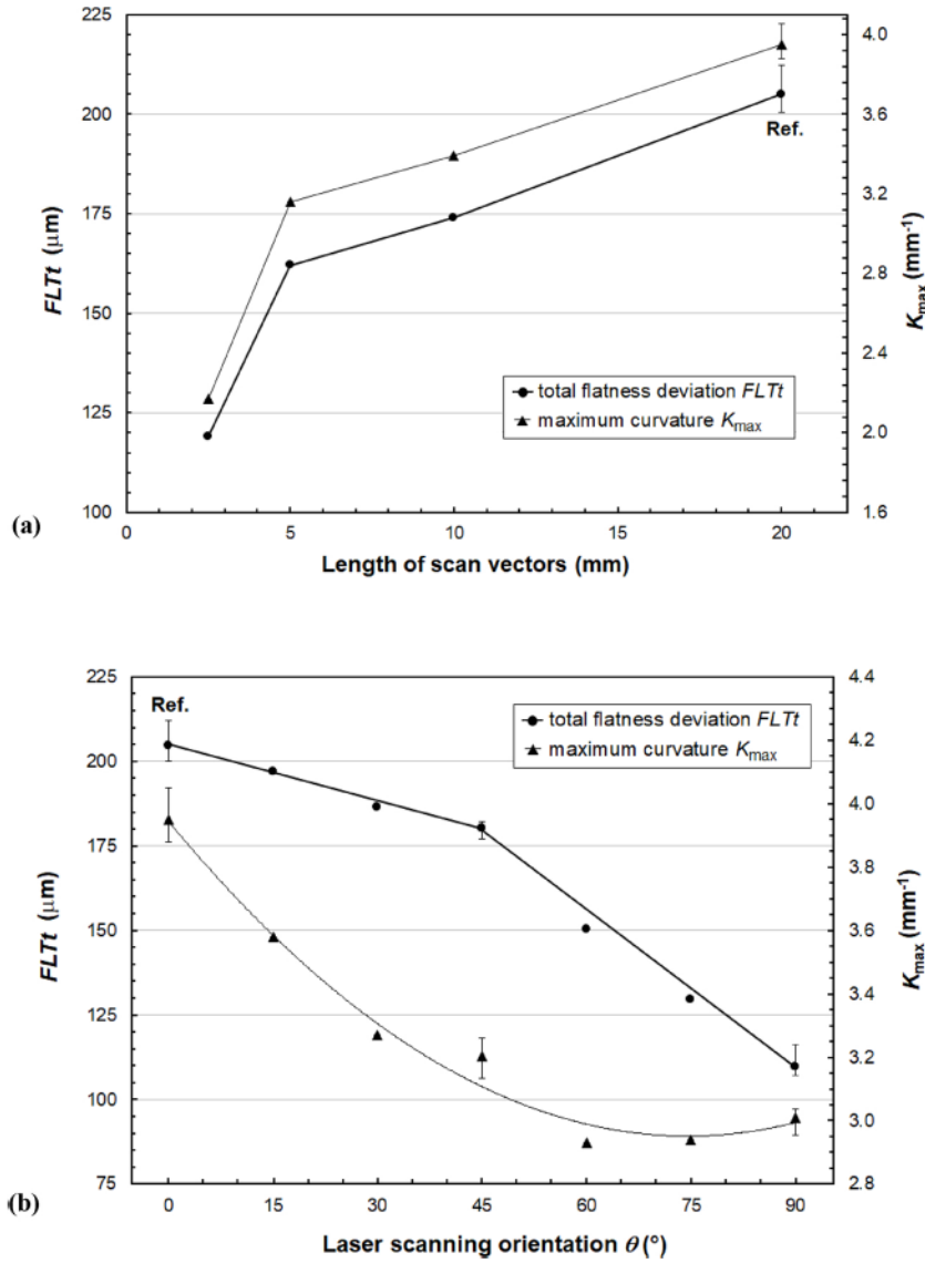
Fig. 9. Effect of (a) the scan vector length L_v and (b) laser scanning orientation \theta on the distortion amplitude determined on conventional bridge specimens by the total flatness deviation ( FLTt ) and the maximum curvature ( K_{\text{max}} ).
