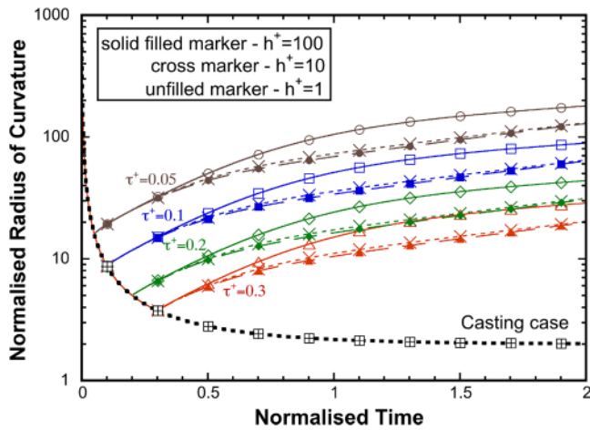
Fig. 18. An example of application of the normalized approach based on transient heat transfer: evolution of the normalized radius of curvature of a slab as a function of the normalized time, for different coefficients of cooling heat transfer h^+ and power switch off time \tau^+ [66].
