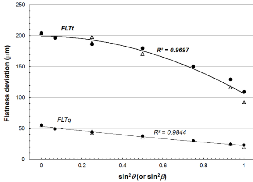
Fig. 10. Relationship between the flatness deviation and the orientation of the scan vectors, for conventional bridge specimens built with the same process parameters ( P = 300 \text{ W} , v = 1800 \text{ mm.s}^{-1} ). [Black markers represent the data resulting from a unidirectional back-and-forth scanning strategy ( \theta ), and white markers the data resulting from a hatch rotation strategy ( \beta )].
