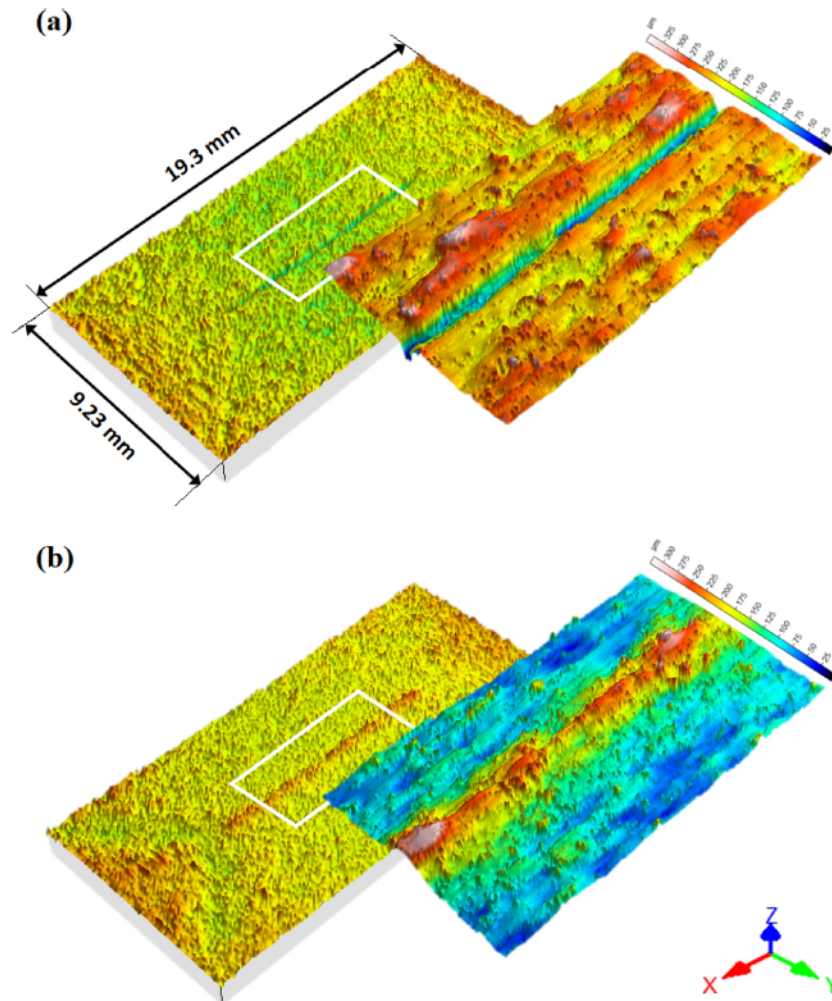
Fig. 6. Surface height maps showing a defect of the central weld bead when the bridge specimen is built using concentric strategies: (a) lack of material (inward scanning direction); (b) swelling of the first weld bead (outward scanning direction).
