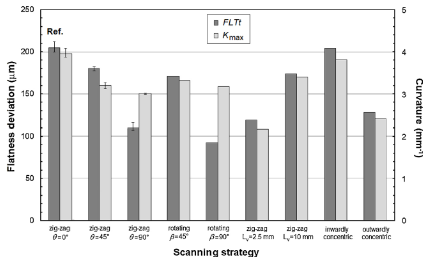
Fig. 7. Comparison of the total flatness deviation and the maximum curvature measured on the conventional bridge specimens built with identical laser power and scanning speed ( P = 300 \text{ W} , v = 1800 \text{ mm} \cdot \text{s}^{-1} ).
