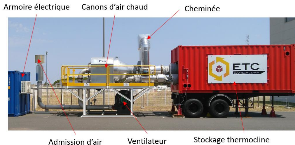
Figure 1: Banc expérimental
