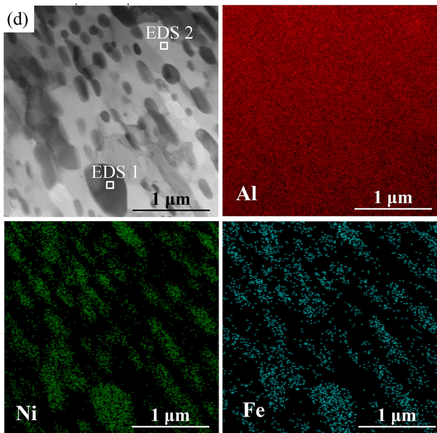
Fig. 5. TEM images of single tracks of Al-Fe-Ni alloys after annealing at (a) 250°C for 20 h, (b) 300°C for 1 h, and (c) 500°C for 1 h, and (d) Fe and Ni distribution maps of the Al-2.5Fe-7.5Ni alloy after annealing at 500°C 1 h.
