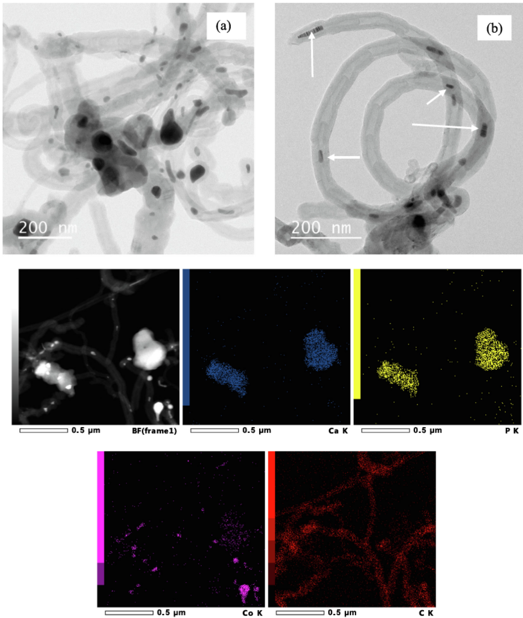
Fig. 11. TEM-EDX analysis of 10Co/HAP_N after DRM reaction at 700 °C and 1.6 bar. Arrows: encapsulated Co particles.
