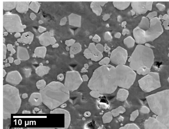
Fig. 1. Microstructure of (a) CuZn40Pb2 brass and (b) W-Cu materials.
