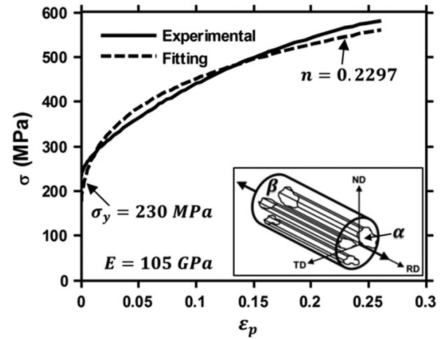
Fig. 4. True stress-true strain curve and elastoplastic parameters of CuZn40Pb2 brass.
