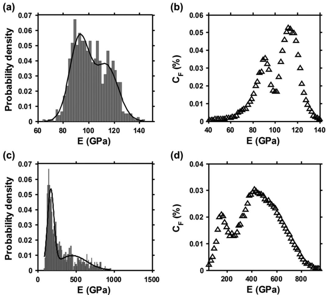
Fig. 16. Comparison between the statistical analysis and the contour analysis applied to the elastic modulus: (a) histogram and (b) contour analysis of CuZn40Pb2 brass; (c) histogram and (d) contour analysis W-Cu.
