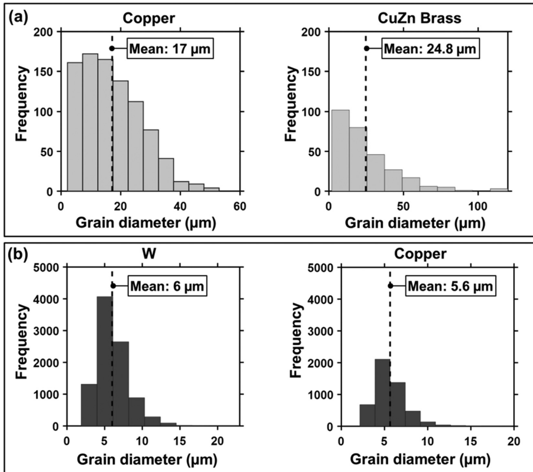
Fig. 3. Distribution of the diameter grain size of each phase for: (a) CuZn40Pb2 brass and (b) W-Cu.
