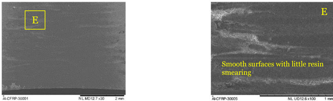
Fig. 12 SEM morphologies of CFRP holes at V_f = 15 mm/min and V_c = 59.346 m/min
