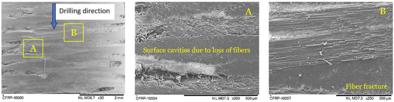
(a) CFRP
