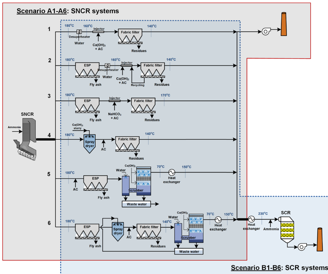
Fig. 2. Flue gas treatment scenarios considered in the study (ESP: electrostatic precipitator; AC: activated carbon). The solid red line denotes the system boundaries for scenarios A1-A6 and dotted blue line the boundaries for scenarios B1-B6).
