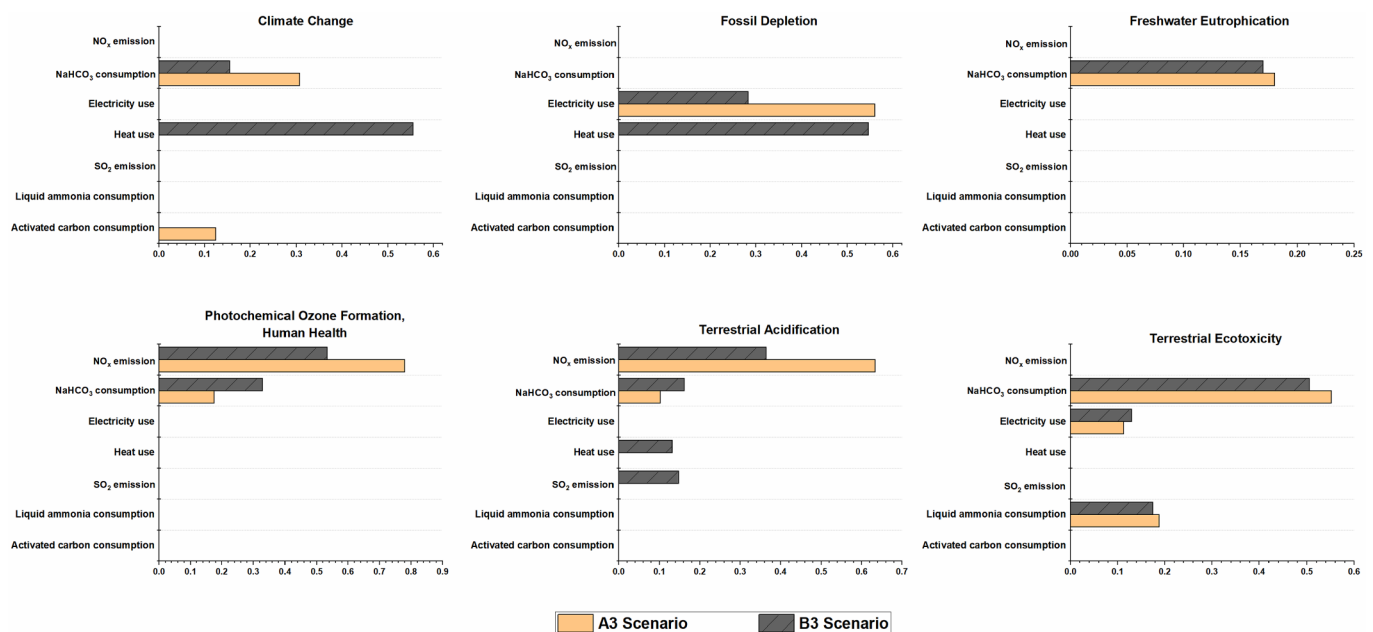
Fig. 4. Sensitivity analysis for input parameters in the A3 and B3 scenarios (Values represent sensitivity ratios (SR) estimated according to Eq. (1). Only SR > 0.1 are presented.)
