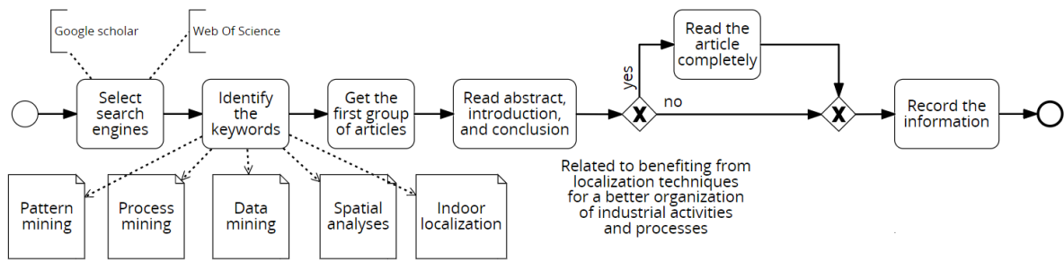
Figure 2: The used approach for analyzing research works related to applying localization techniques for a better organization of processes and activities in different industries.
