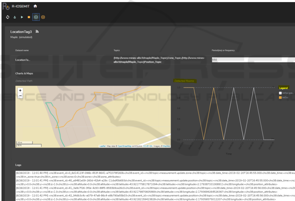
Figure 7: An illustration of the interpretation procedure.
