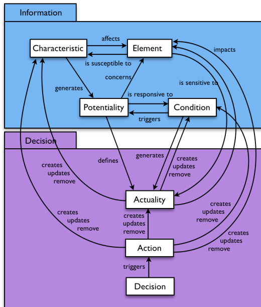
Figure 8. Potentially management metamodel.
