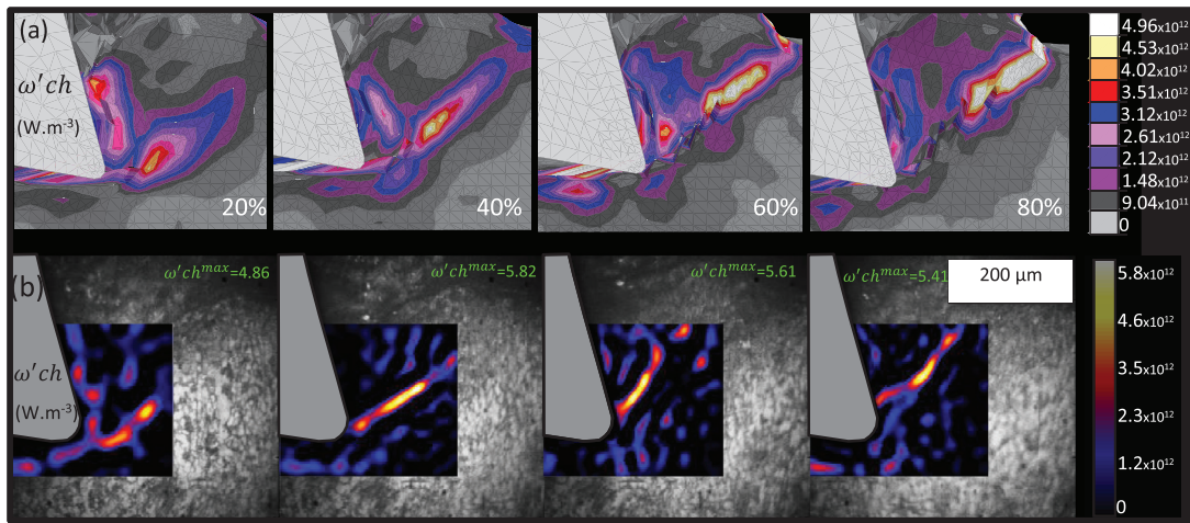
Fig. 13. The evolution of the intrinsic dissipation during chip segment formation in the case of Test 1. (a) numerical results (b) experimental results.
