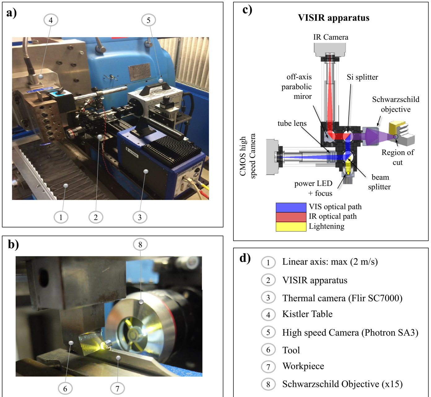
Fig. 1. Orthogonal cutting experimental setup: a) linear actuator, cutting tool and optical apparatus b) close up view of the cut c) VIS-IR apparatus detailed design d) nomenclature.
