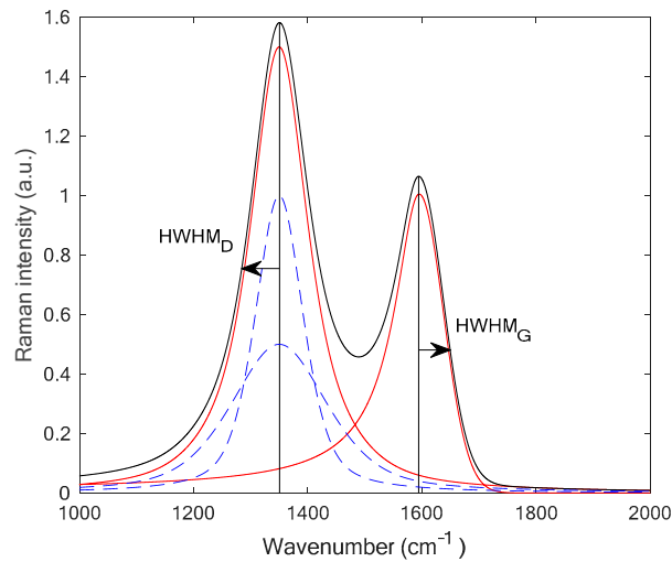
Figure 1. Typical Raman spectrum (black line) for a disordered carbon showing the principle of hand-made measurement of the half width at half maximum ( HWHM ). HWHM_D ( HWHM_D ) is for the D band (G band respectively). The G and D band contributions are plotted in red. The dotted blue reports the D band decomposition in two Voigt sub-bands (same wavenumber).
