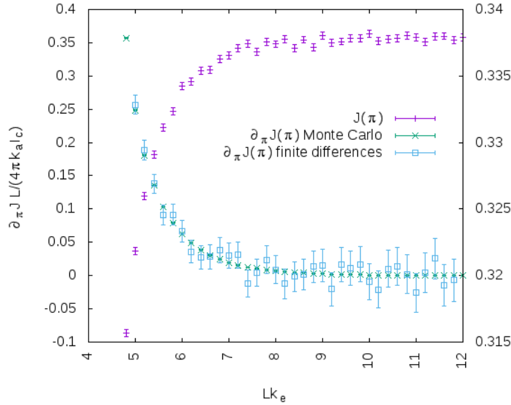
Figure 4. Absorbed radiative intensity density J(\pi) and its sensitivity \partial_\pi J(\pi) to the normal transformation of the \mathcal{R}(\pi) boundary. The phase function in a semi-transparent medium is isotropic p_{\vec{U}}(\vec{u}_i) = \frac{1}{4\pi} and the probability density function of scattering extinction is p_\Sigma(l_i) = k_s \exp(-k_s l_i) . Cavity dimensions are set by a variation \delta L of L influencing the optical thickness k_e L . Single scattering albedo is uniform on the cavity \frac{k_s}{k_e} = 0.5 . Estimations of the absorbed radiative intensity density and its sensitivity are obtained for 2.10^6 realizations N of the corresponding Monte-Carlo weight function.
