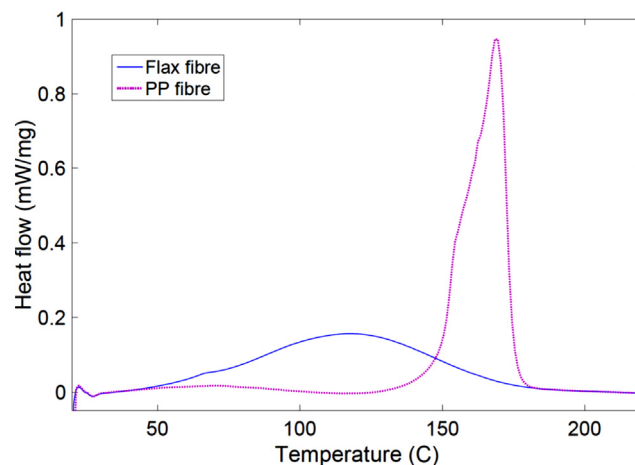
Fig. 2. DSC heating scan for the first heating cycle of PP fibres and flax fibres. (For interpretation of the references to colour in this figure legend, the reader is referred to the web version of this article.)
