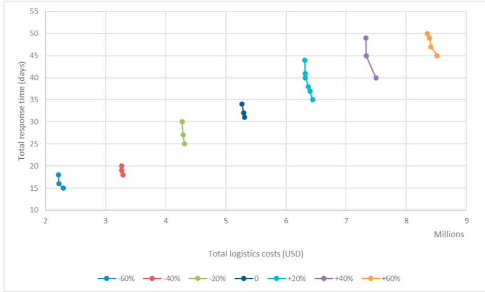
Fig. 13. Impact of changing relief items weights.
