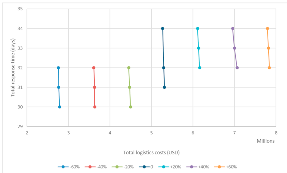
Fig. 12. Impact of changing air transportation costs.
