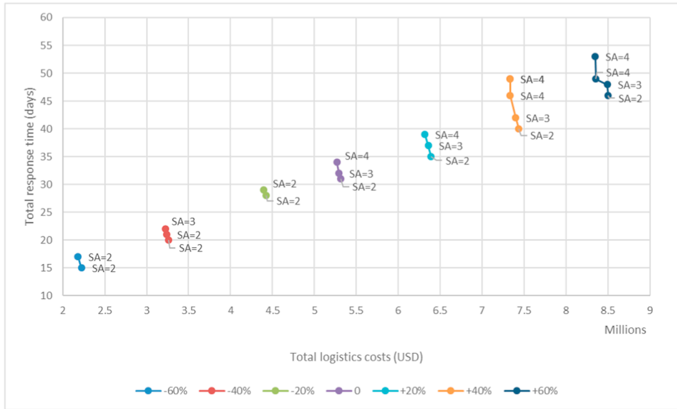
Fig. 7. Impact of changing the demands.
