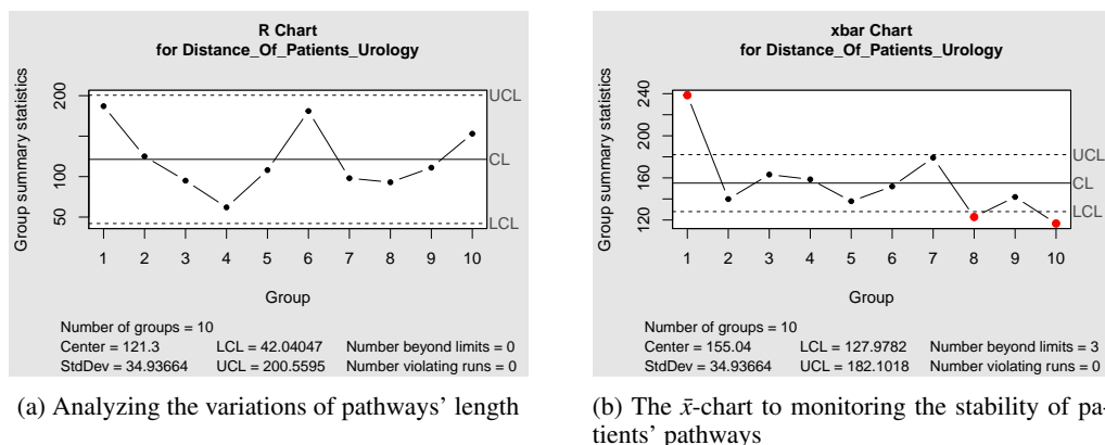
Figure 4: Control charts analysis related to the distance of pathways.
