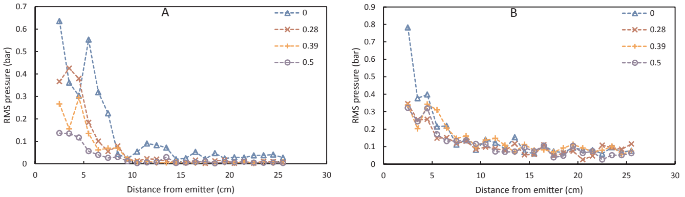
Fig. 15. Effect of the solid hold-up on the axial evolution of the RMS pressure calculated over different spectrum parts – case of plastic particle suspension (2 mm diameter), emitted US power = 150 W – (A) Fundamental frequency – (B) Broad-band noise.
