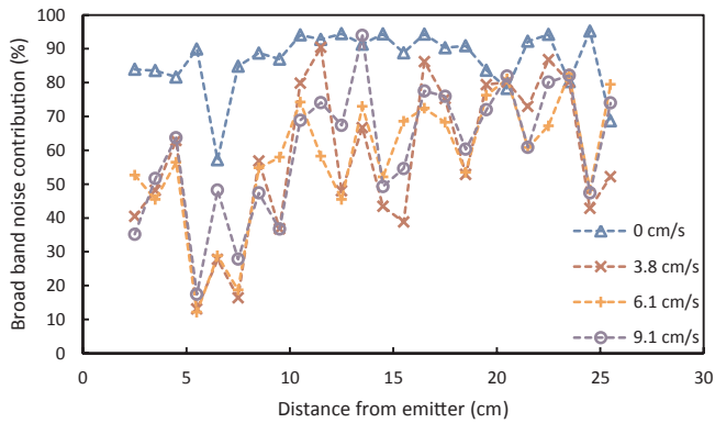
Fig. 13. Effect of liquid velocity on the axial evolution of the broad-band noise contribution – case without solid, emitted US power = 150 W.
