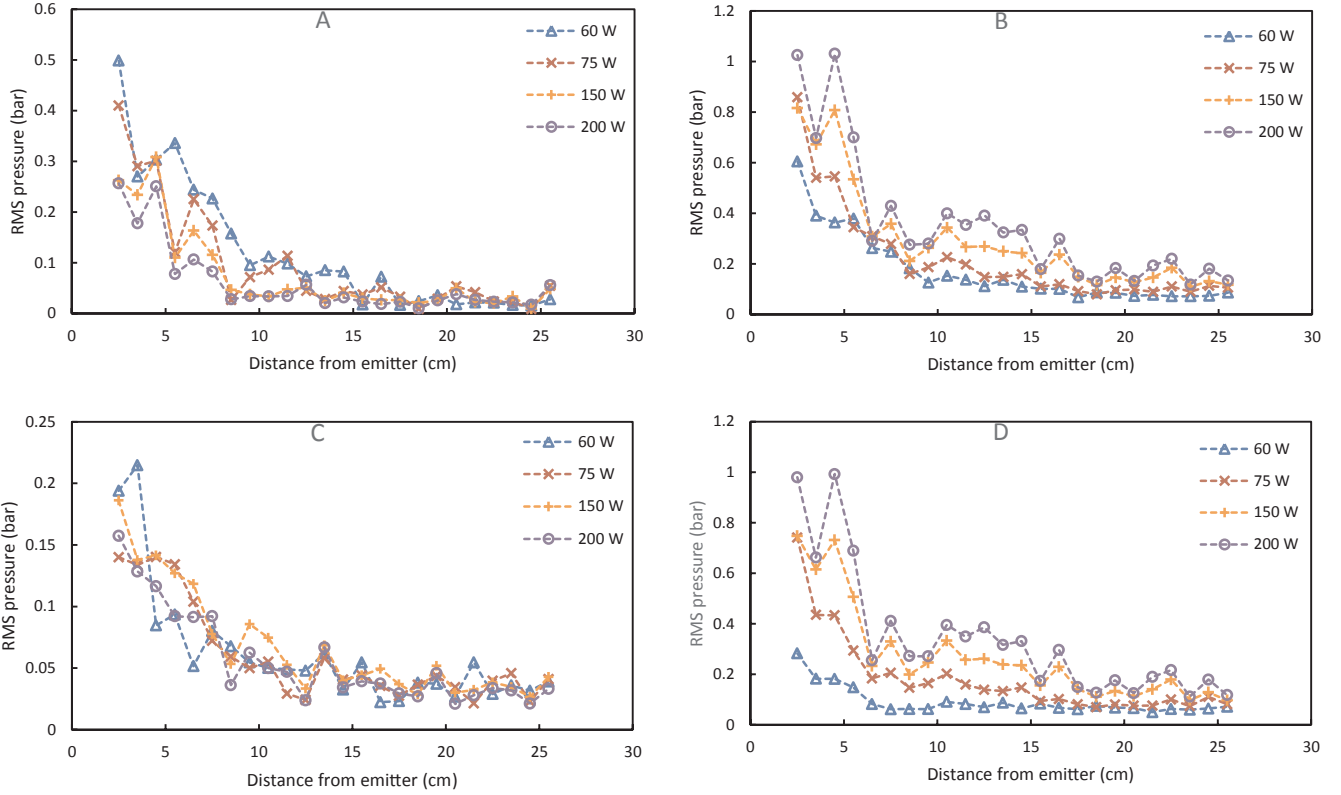
Fig. 10. Effect of emitted US power on the axial evolution of the RMS pressure calculated over different spectrum parts – case of non-flowing liquid – (A) Fundamental frequency– (B) Total spectrum – (C) (sub/ultra) harmonics – (D) Broad-band noise.
