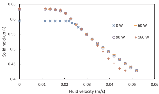
Fig. 8. Fluidization of 2 mm glass beads under power ultrasound with decreasing flow only – Solid hold-up.
