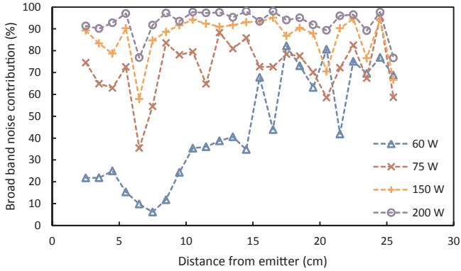
Fig. 11. Effect of emitted US power on the axial evolution of the broad-band noise contribution – case of non-flowing liquid.
