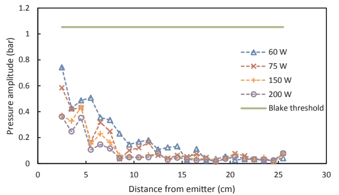
Fig. 9. Effect of emitted US power on the axial evolution of the pressure amplitude at the fundamental frequency (case of non-flowing liquid) and comparison with the value of the Blake threshold calculated for 5 \mu m diameter bubbles.
