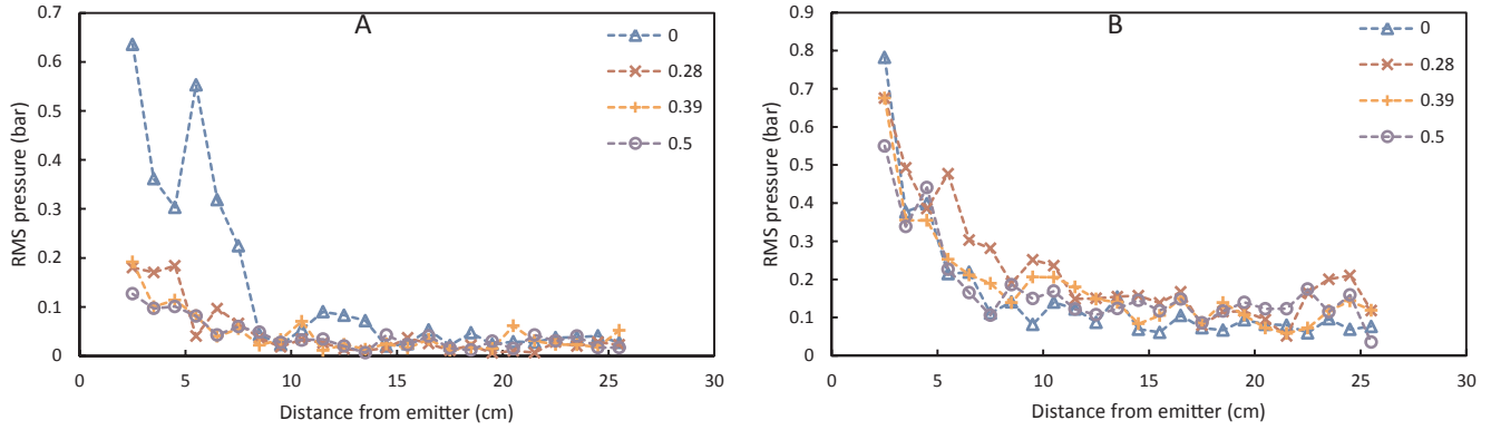
Fig. 14. Effect of the solid hold-up on the axial evolution of the RMS pressure calculated over different spectrum parts – case of glass particle suspension (2 mm diameter), emitted US power = 150 W – (A) Fundamental frequency – (B) Broad-band noise.
