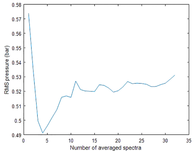
Fig. 5. Effect of the number of averaged spectra on RMS pressure of the total spectrum.
