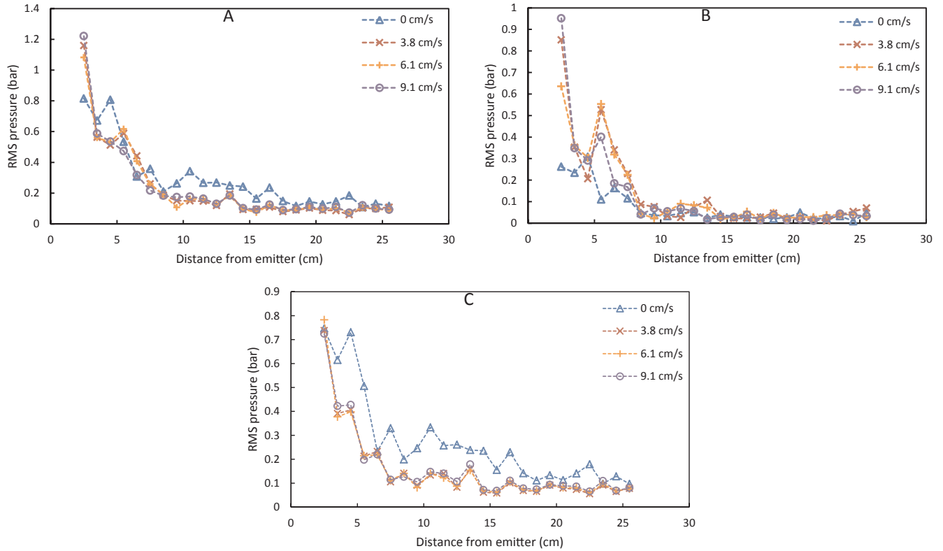
Fig. 12. Effect of liquid velocity on the axial evolution of the RMS pressure calculated over different spectrum parts – case without solid, emitted US power = 150 W – (A) Total spectrum – (B) Fundamental frequency – (C) Broad-band noise.
