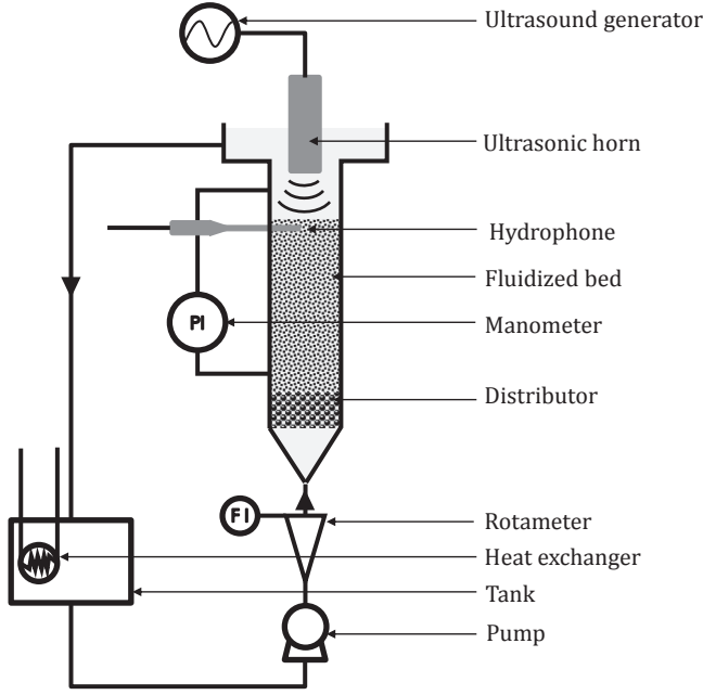
Fig. 1. Experimental setup.
