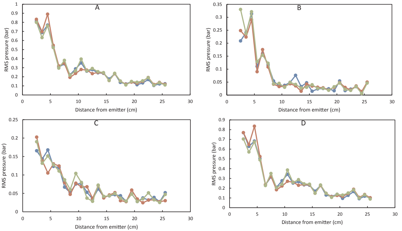
Fig. 6. Repeatability of the RMS pressure vs. axial distance from the emitter curves (emitted US power = 150 W, no solid and no liquid flow, 3 repetitions): (A) Total spectrum, (B) Fundamental, (C) (sub/ultra) Harmonics and (D) Broad-band noise.
