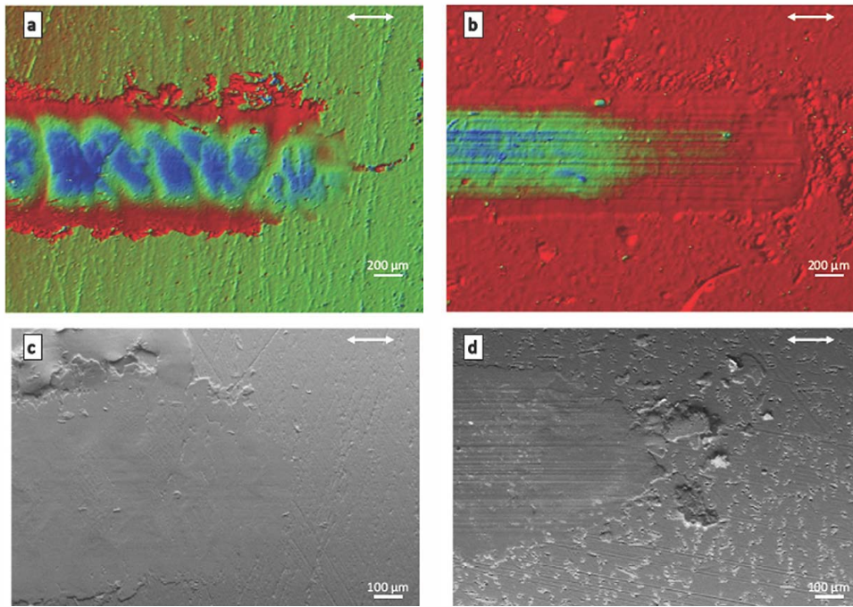
Fig. 4. Profilometry images (a and b) and SEM images (c and d) of worn surfaces for tests during 1500 s; pure PEEK (a and c), PEEK-GF30 (b and d). \longleftrightarrow : sliding direction.
