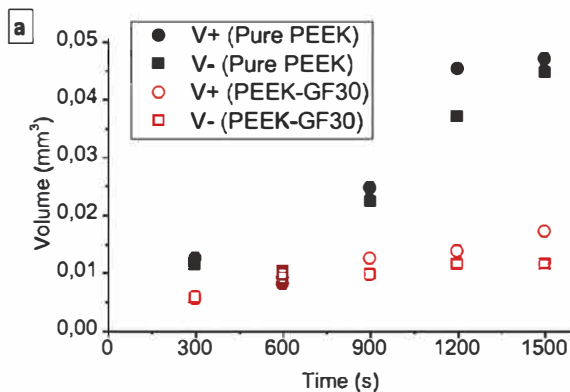
Fig. 3. Evolution for PEEK and PEEK-GF30 of a) V^+ and V^- and b) V_{\text{dam}} and V_{\text{wear}} .
