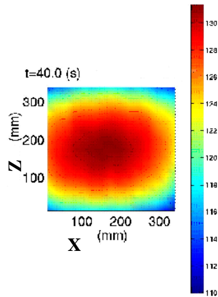
Figure 8- Calculated temperatures
