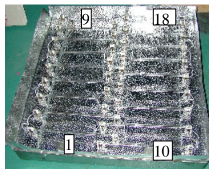
Figure 3- Infrared oven designed with numerical simulations
