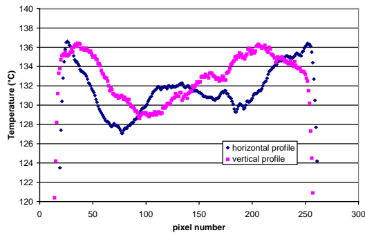
Figure 7- Temperature profiles
