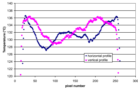
Figure 7- Temperature profiles
