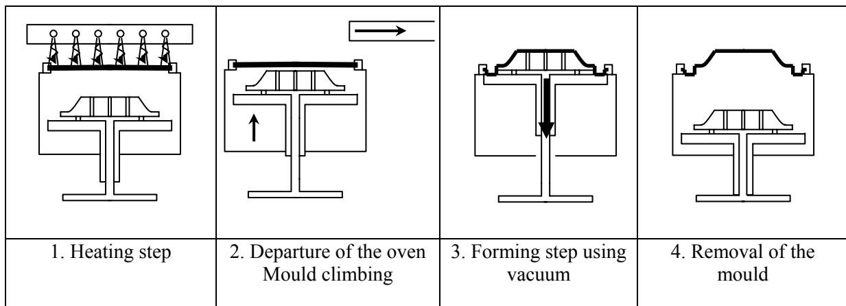
Figure 1 – The different steps of thermoforming
