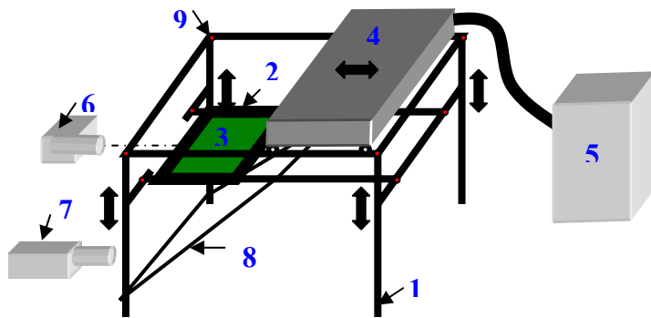
Figure 4 – Experimental infrared heating set-up plan
