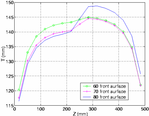
Figure 12 – Front surface temperature versus z
