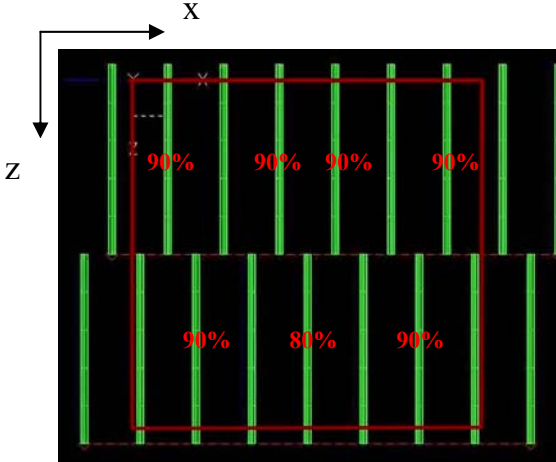
Figure 17 – 80 mm with power regulation
