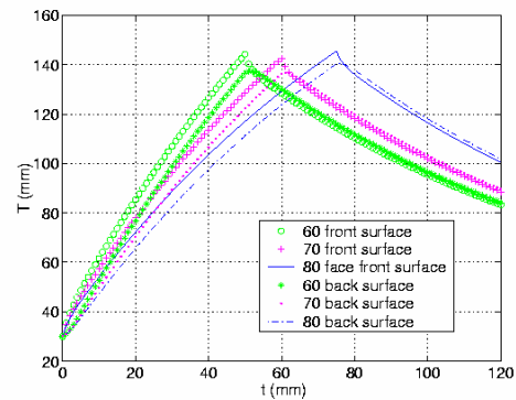
Figure 9 – Temperature versus heating time
