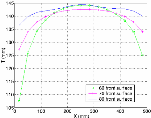
Figure 10 – Front surface temperature versus x
