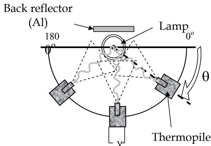
Figure 2 – Experimental set-up used in order to measure spatial directivity
