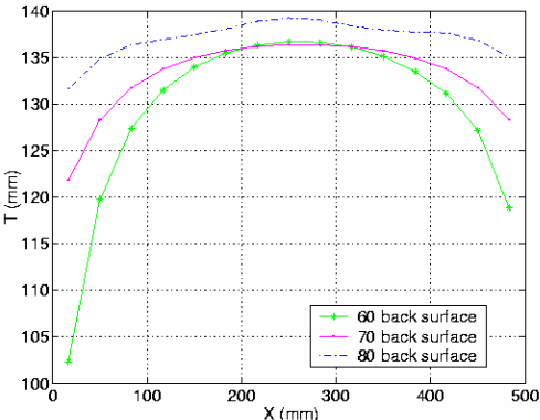
Figure 11 – Back surface temperature versus x
