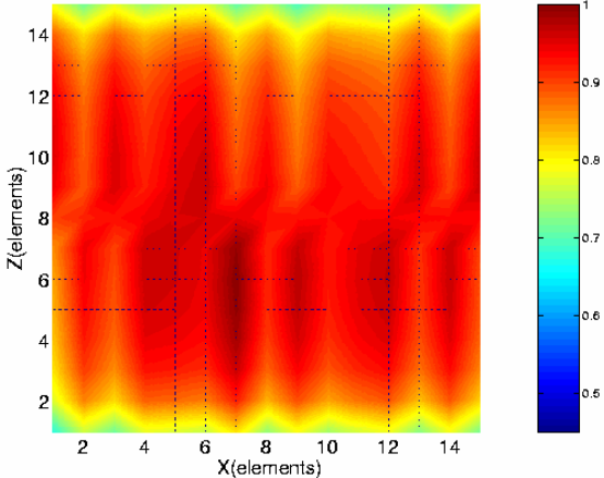
Figure 18 – 80 mm interval distribution energy criterion with power regulation
