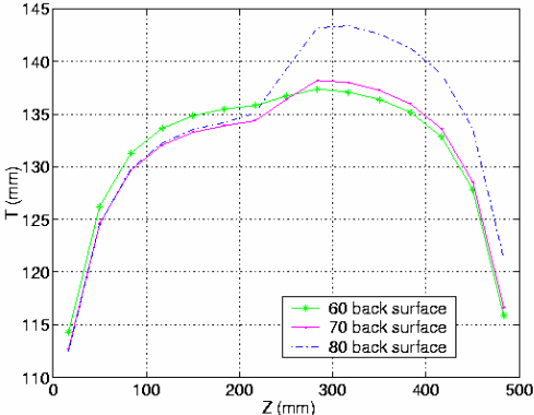
Figure 13 – Back surface temperature versus z
