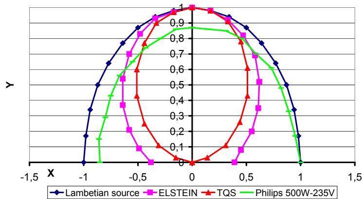
Figure 3 – Infrared heater's directivity
