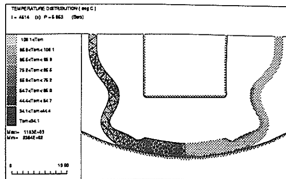
Fig. 3 Temperature distribution
