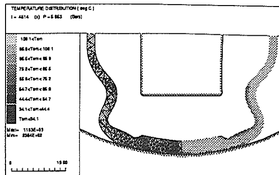
Fig. 3 Temperature distribution
