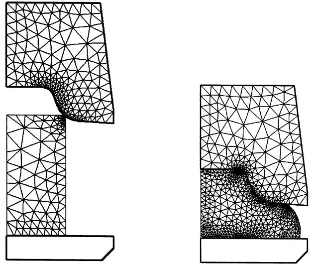
Fig. 7. Initial and final configuration of the finite-element simulation.
