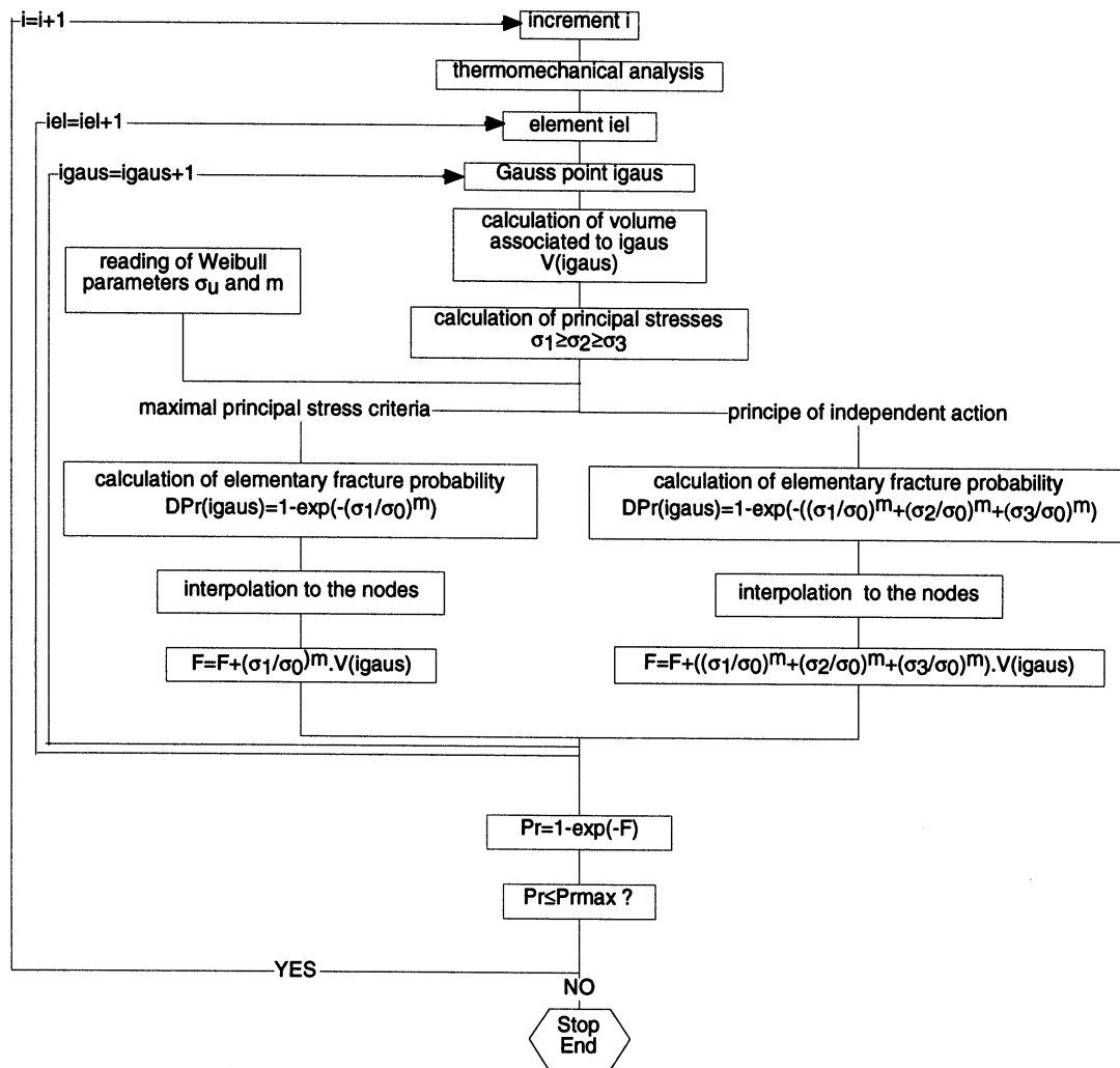
Fig. 1. Computational elements of the failure-prediction routine.
