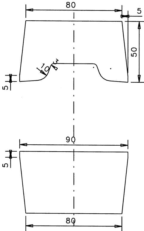
Fig. 6. Geometry of the tools (dimensions: mm).
