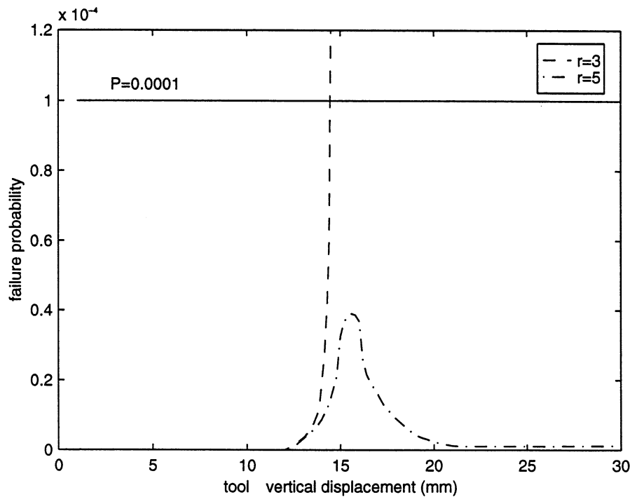
Fig. 8. Evolution of the fracture probability of the upper tool as a function of its displacement, for two different engraving concave fillet radii.
