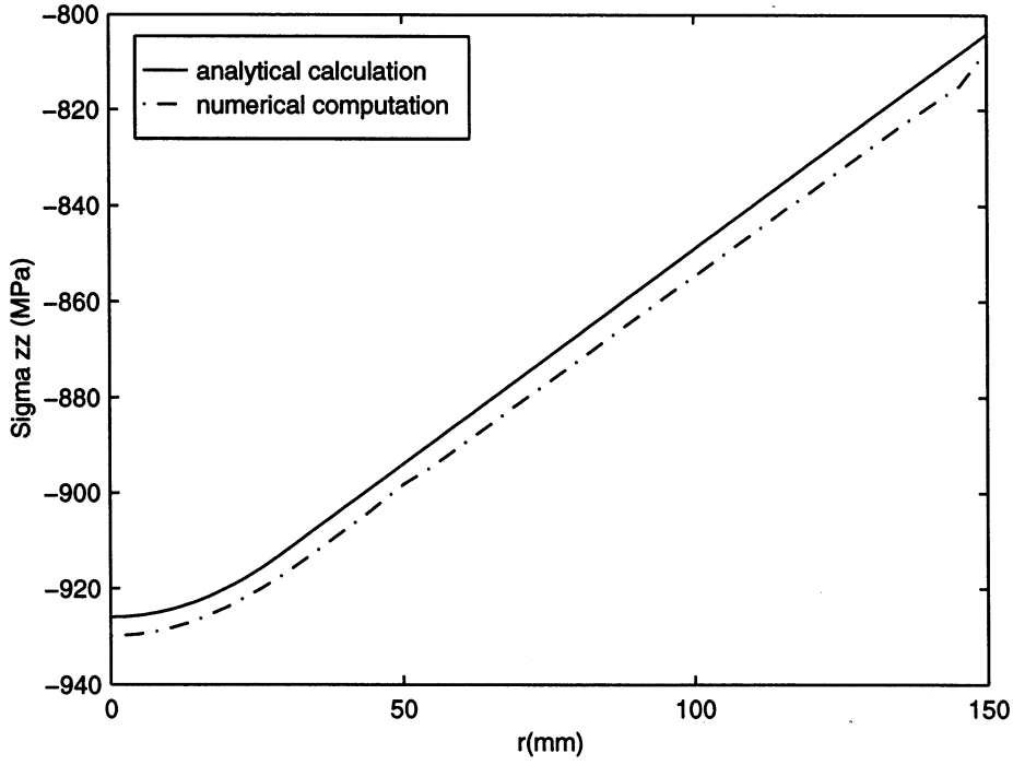
Fig. 3. Evolution of the stress \sigma_{zz} as a function of the radius r .
