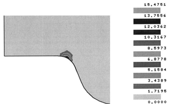
Fig. 9. Local risk of rupture (%) of the upper tool around the engraving fillet radius.
