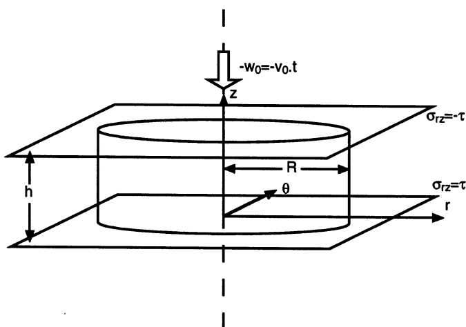
Fig. 2. A cylindrical workpiece pressed between two planes with uniform friction.
