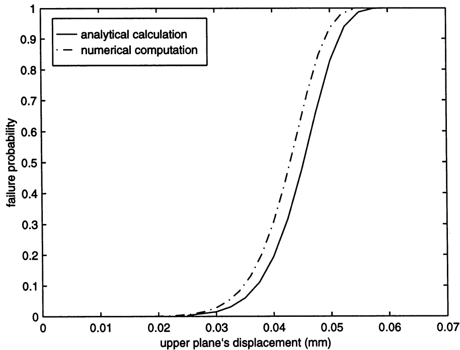
Fig. 4. Evolution of the failure probability of the cylinder as a function of the displacement of the upper tool.
