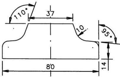
Fig. 5. Final geometry of the forged piece (dimensions: mm).
