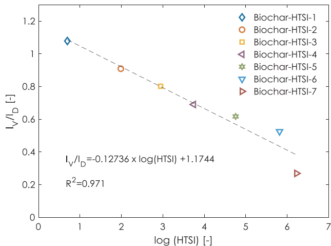
Fig. 6. I_V/I_D as a function of \log(HTSI) .
