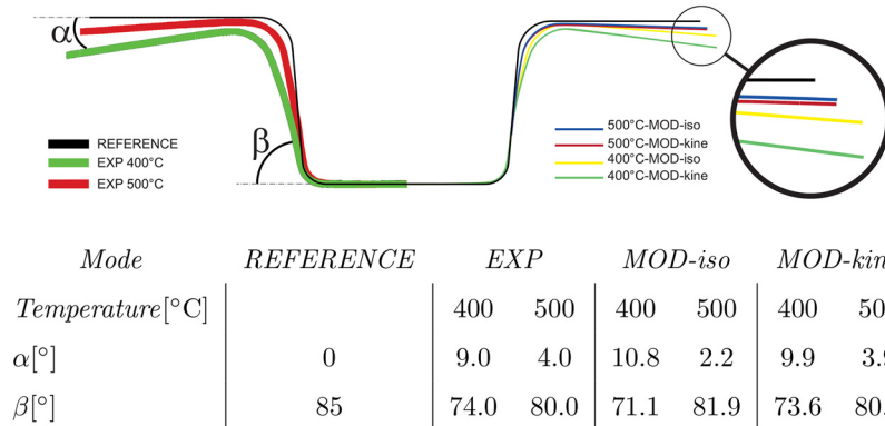
Fig. 15. Springback comparison between reference, experimental and simulated omega test.
