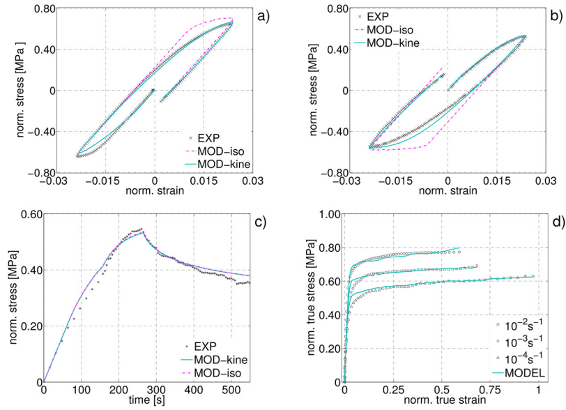
Fig. 11. Graphs for true stress–true strain for RD, at 500 °C: push-pull at 10^{-2} \text{ s}^{-1} strain rate (a), pull-push at 10^{-4} \text{ s}^{-1} strain rate (b), relaxation test at 10^{-4} \text{ s}^{-1} first strain rate (c), uniaxial tensile test at 10^{-2} \text{ s}^{-1} , 10^{-3} \text{ s}^{-1} and 10^{-4} \text{ s}^{-1} strain rate (d).
