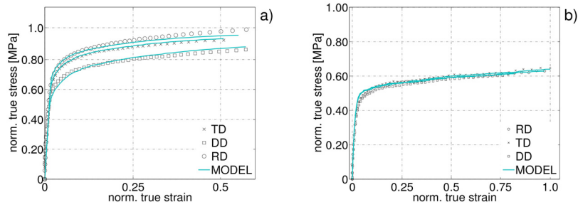
Fig. 12. Graphs for true stress–true strain at 10^{-4} \text{ s}^{-1} strain rate and for RD, DD, TD and model at: 400 °C (a) and 500 °C (b).
