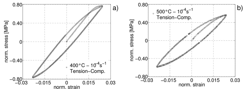
Fig. 7. Stress vs strain of Ti-6Al-4V titanium alloy for cyclic test at 400 \text{ °C} (a) and 500 \text{ °C} (b).
