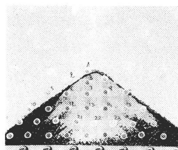
Fig. 2. Test rig developed by Massol-Chaudeur et al. (2003)[4] for evaluating segregation of powder mixtures
