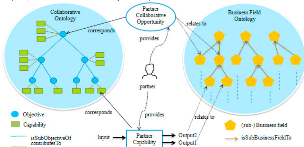
Fig. 3. The link between partners' inputs to the two ontologies.
