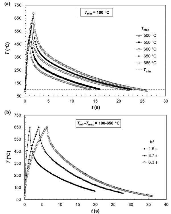
Fig. 1. Temperature-time cycles applied in thermal fatigue experiments: (a) with various maximum temperatures T_{\max} , (b) with various heating times ht .
