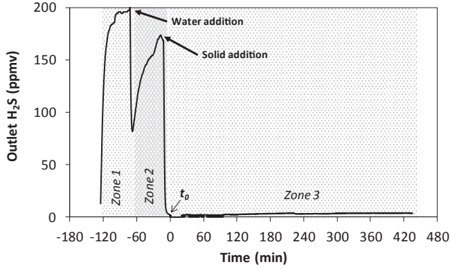
Fig. 2. Example of profile of H_2S concentration at the outlet of reactor. Conditions: gas flow rate of 100 \text{ mL min}^{-1} , inlet concentration of H_2S of 200 ppmv, 100 mL of suspension, 5 wt% of solid using APC as reactive sorbent, room temperature and pressure.
