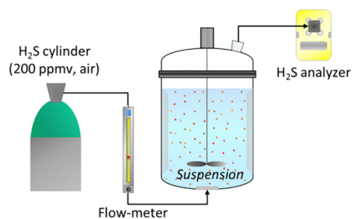
Fig. 1. Tri-phasic system for H 2 S removal at laboratory scale.
