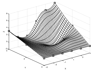
Figure 2. Surface for z=f(x,y)
