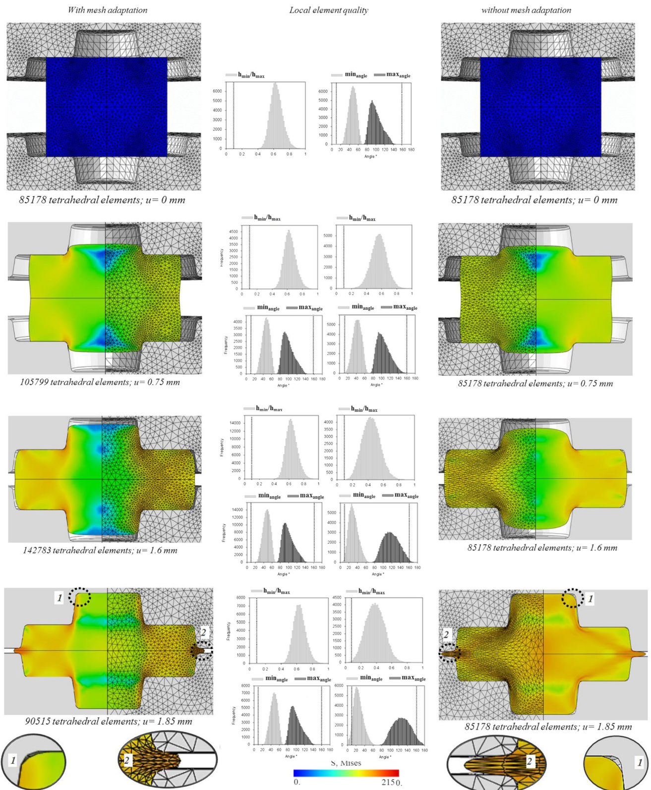
Fig. 16 Meshes at different tool displacement in the left with mesh adaptation and in the right without mesh adaptation
