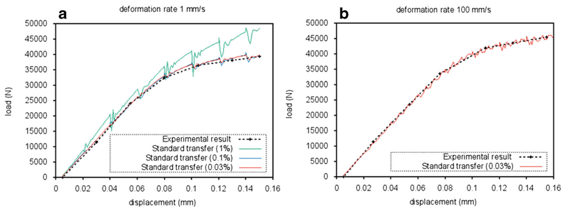
Fig. 12 Comparison of load–displacement curves of mechanical tests using different deformation rate: 1 mm/s and 100 mm/s
