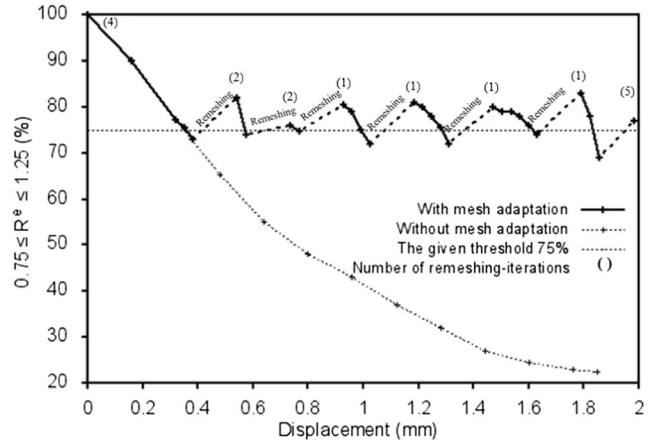
Fig. 17 The evolution of the percentage of optimal element with and without mesh adaptation
