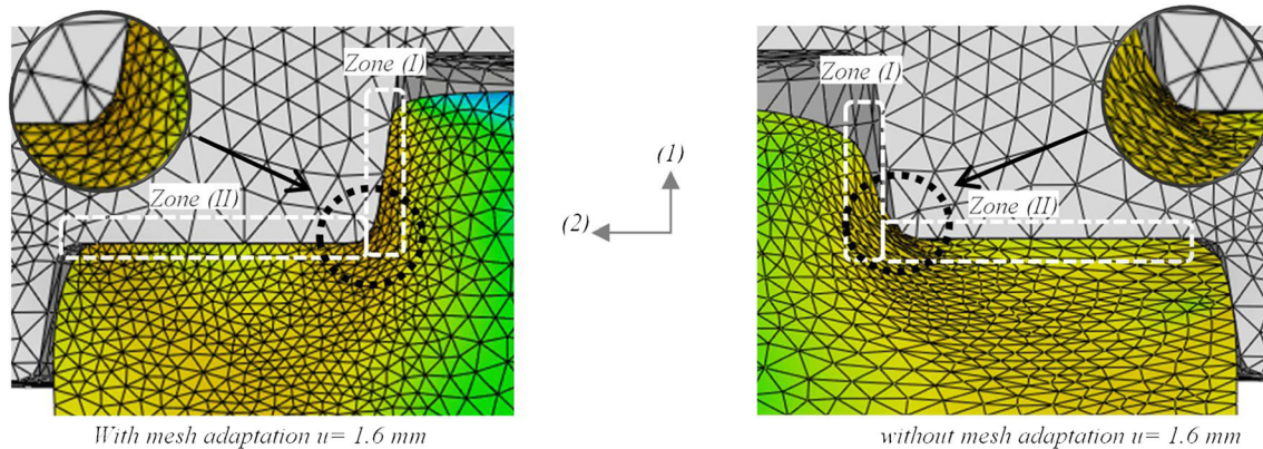
Fig. 19 The effect of mesh-distortion on the geometry of the workpiece
