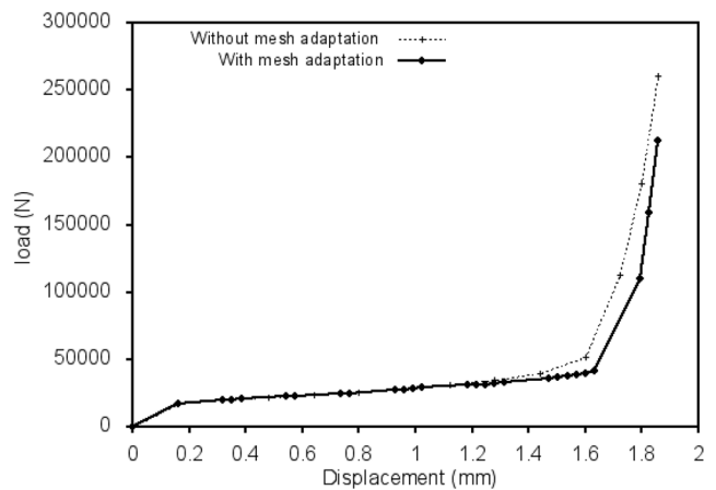
Fig. 18 Comparison of load–displacement curves of forming tests with and without mesh adaptation
