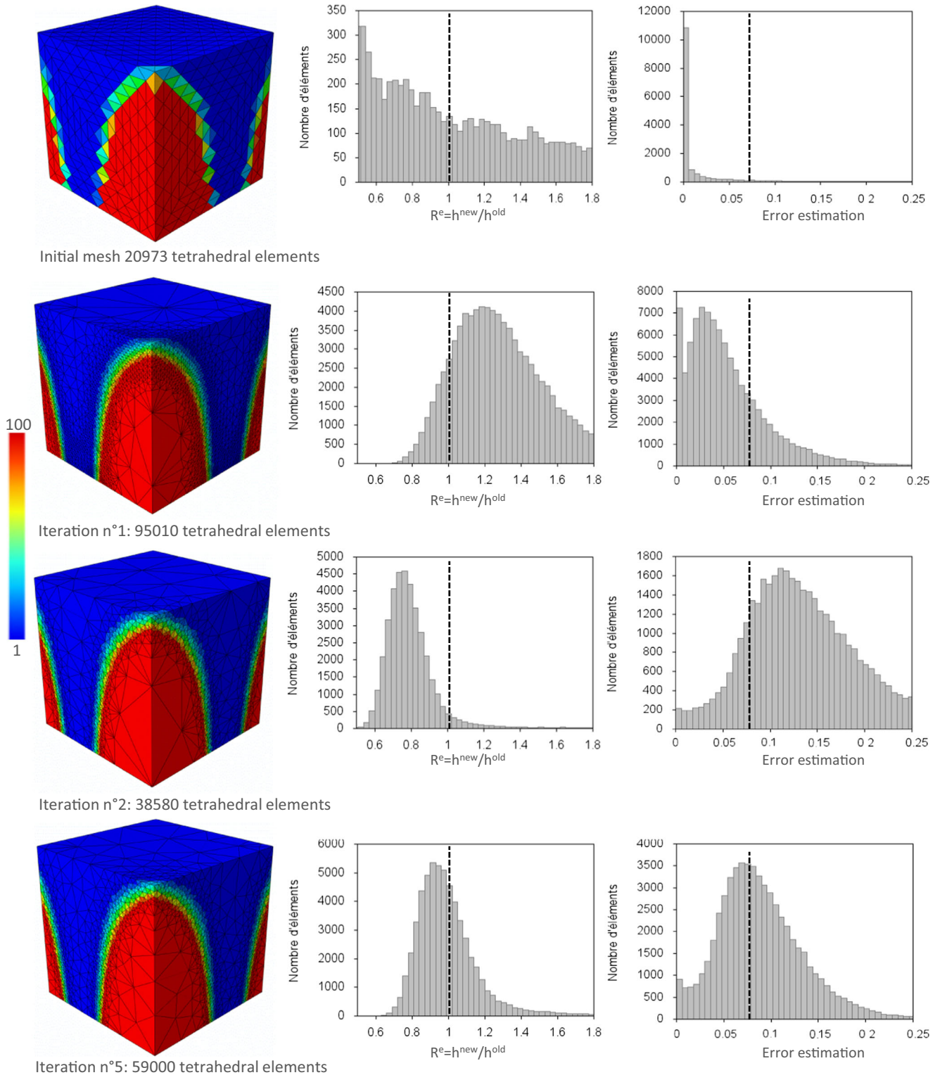
Fig. 6 Iso values of the tested analytical function: f_1(x,y,z) mesh size coefficient: R^e , and local error estimation for each remeshing step
