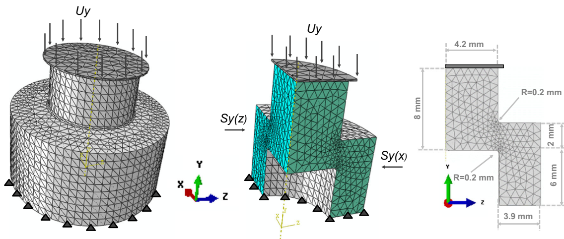
Fig. 10 Geometry and boundary conditions of the specimens used in shear test
