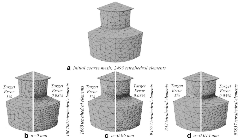
Fig. 11 Meshes at different instants with different targets errors
