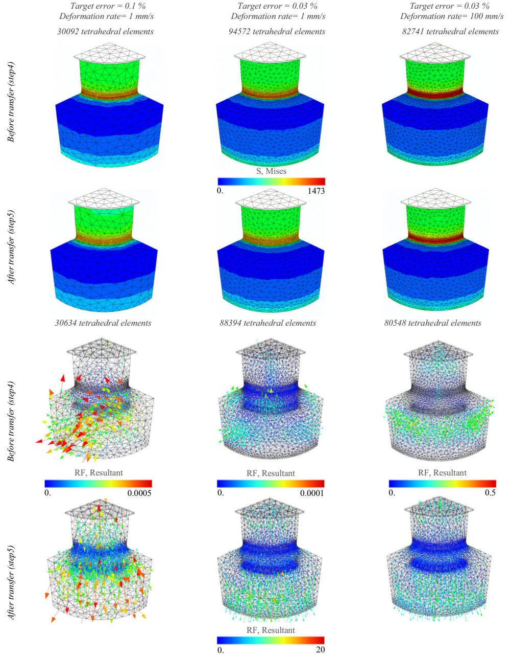
Fig. 13 The evolution of the von Mises stress and the nodal force caused by stress smoothing before and after transfer at the same displacement u = 0.08 mm
