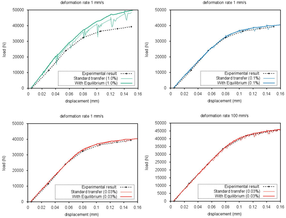
Fig. 14 Comparison of load–displacement curves of mechanical tests before and after equilibrium
