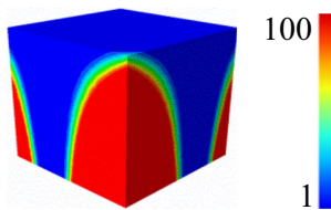
Fig. 5 The analytic values of the function f_1(x,y,z)
