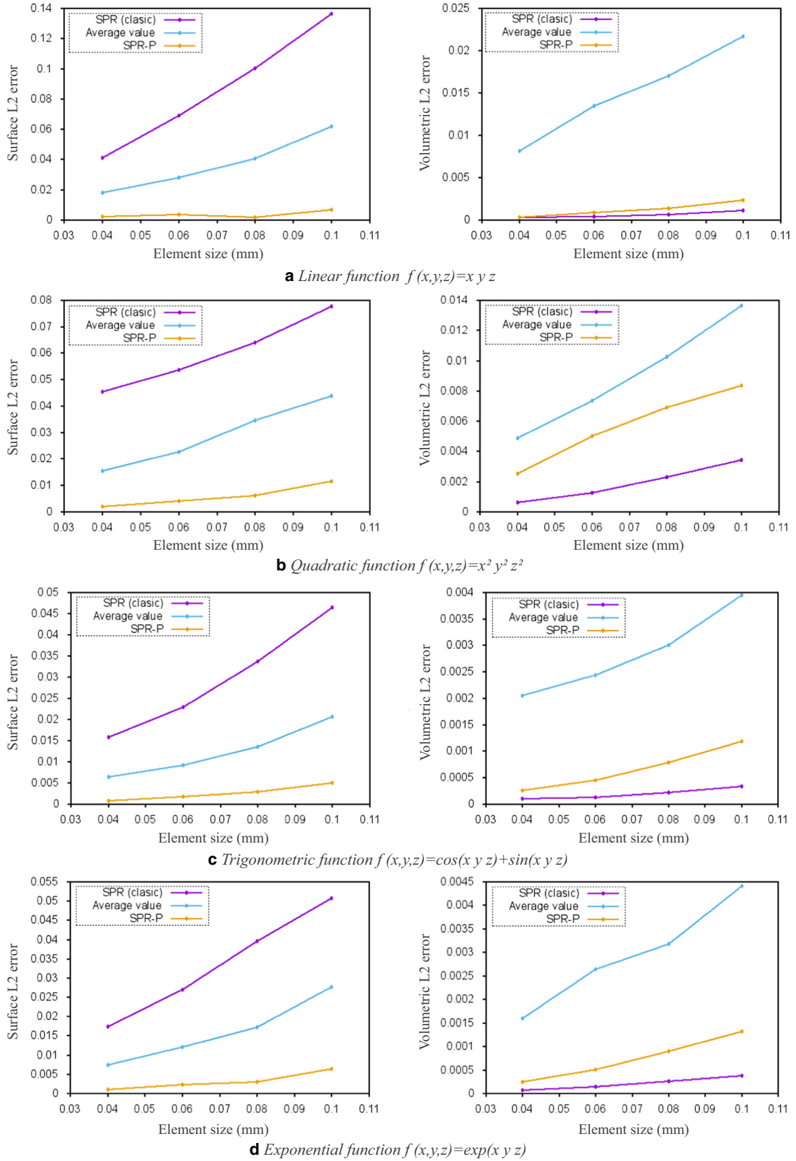
Fig. 7 Comparison between some indirect transfer operators with linear, quadratic, trigonometric and exponential functions
