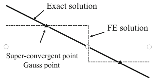
Fig. 2 Approximated values and exact solution
