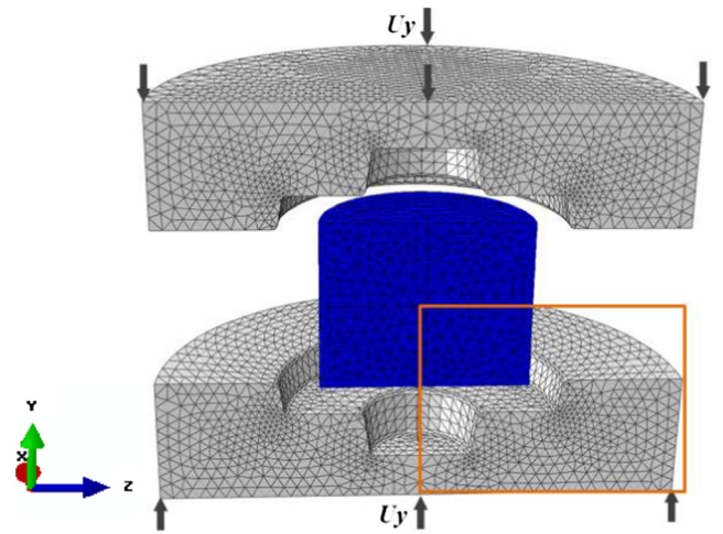
Fig. 15 Geometry, boundary conditions, and initial finite elements discretization
