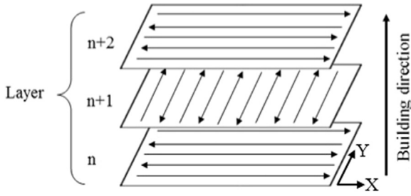
Fig. 3. Laser scanning strategy used in SLM experiments.
