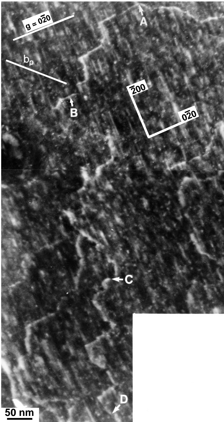
Figure 2. Post-mortem dark-field image of a specimen strained at 2% at 170°C. The diffraction vector is g = 0\bar{2}0 from the aluminium matrix. Projections in the observation plane of the \langle 100 \rangle directions are indicated.
