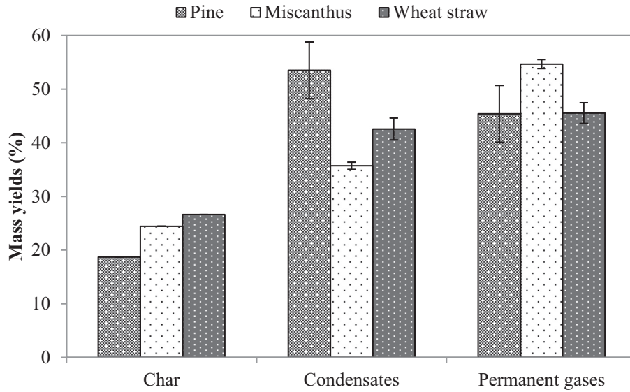
Fig. 6. Mass yields ( daf ) of the oxidative pyrolysis products from different biomasses, 0.022 \text{ kg m}^{-2} \text{ s}^{-1} air flux.
