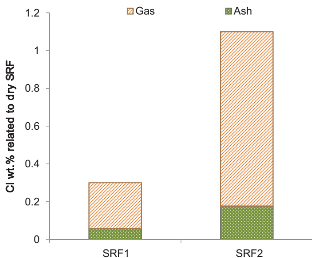
Fig. 12. Distribution of chlorine in the gas phase and the solid residual phase after the oxidation tests at 800 °C of both SRFs.
