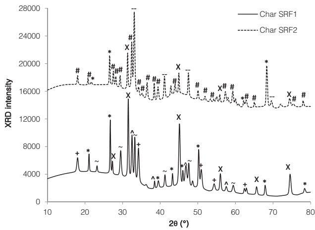
Fig. 9. XRD patterns for both chars produced after pyrolysis tests of SRFs. (x): diffraction peaks of NaCl, (+) diffraction peaks of Ca(OH) 2 et (*): diffraction peaks of SiO 2 , (~): diffraction peaks of Ca 3 Al 2 O 6 , (#): diffraction peaks of Ca 2 SiO 4 , ('): diffraction peaks of K 2 MgSiO 4 , and (-): diffraction peaks of CaTiO 3 .
