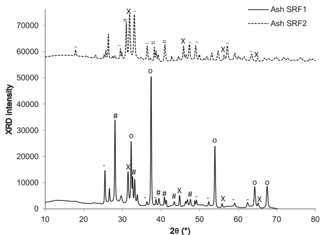
Fig. 13. XRD patterns for both ashes produced after oxidation tests of SRFs. (x): diffraction peaks of NaCl, (°): diffraction peaks of \text{Ca}_3\text{Fe}_2(\text{SiO}_4)_3 , (=): diffraction peaks of \text{FeSi}_4\text{P}_4 , (o): diffraction peaks of CaO, (#): diffraction peaks of \text{Ca}_2\text{SiO}_4 and (-): diffraction peaks of \text{CaSO}_4 .
