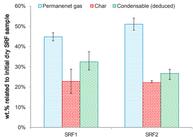
Fig. 5. Product yields of SRFs pyrolysis.
