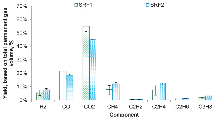
Fig. 11. Permanent gas composition of SRFs oxidation.
