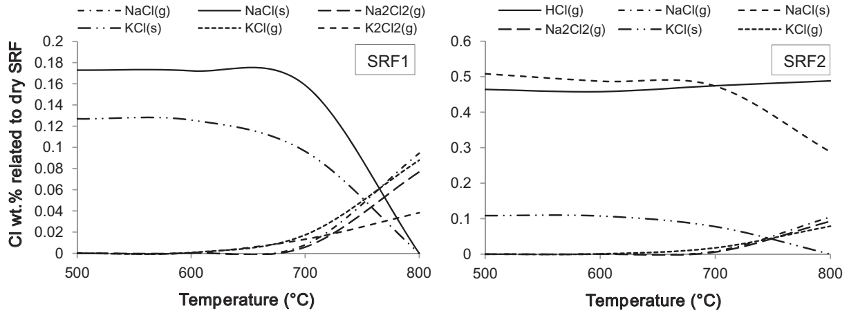
Fig. 8. Percentage of HCl, NaCl, KCl, Na 2 Cl 2 and K 2 Cl 2 based on dry SRF in both gaseous and solid phases calculated with FactSage.
