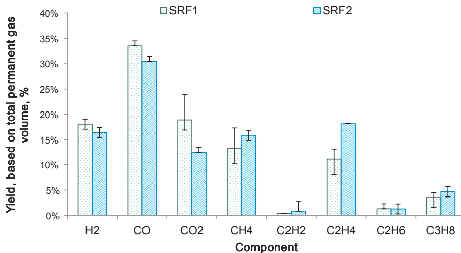
Fig. 6. Permanent gas composition of SRFs pyrolysis.
