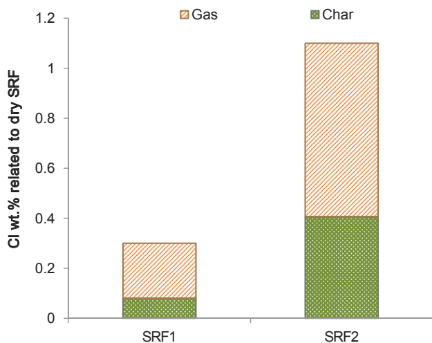
Fig. 7. Distribution of chlorine between the gas phase and the solid residual phase after the pyrolysis tests at 800 °C of both SRFs.
