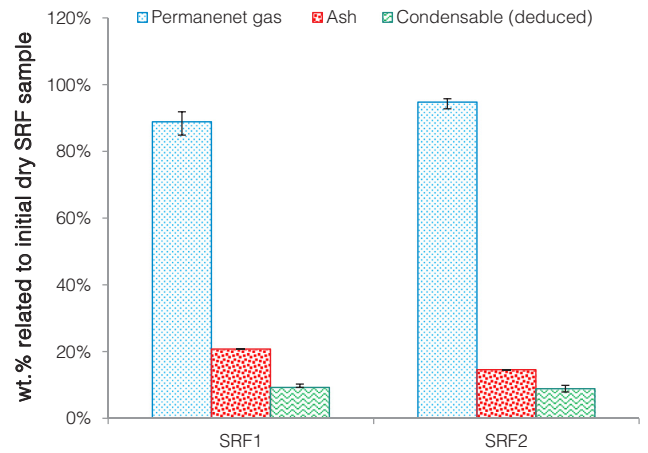
Fig. 10. Product yields of SRFs oxidation.
