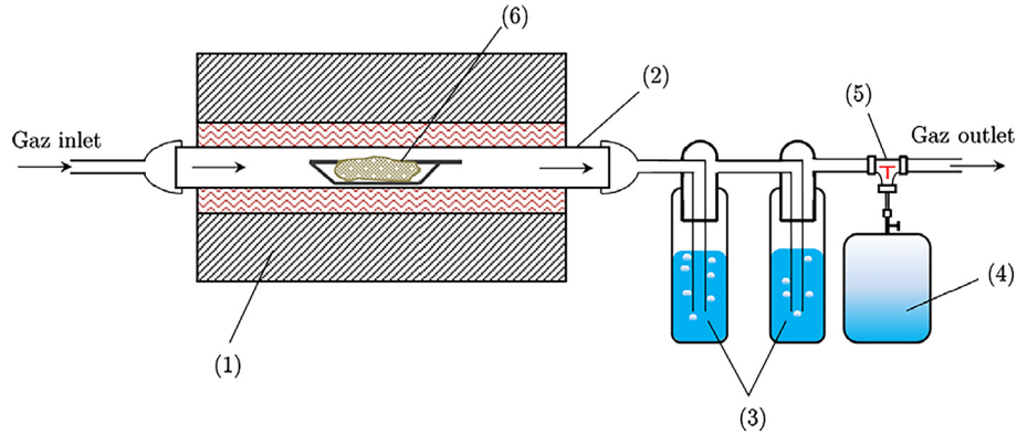
Fig. 4. Diagram of experimental device. (1) Furnace; (2) reactor; (3) isopropyl alcohol impingers; (4) gas sampling bag; (5) three-way valve; (6) crucible with SRF sample.
