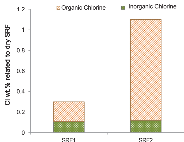
Fig. 3. Chlorine content and its distribution between organic and inorganic chlorine for both studied SRFs.
