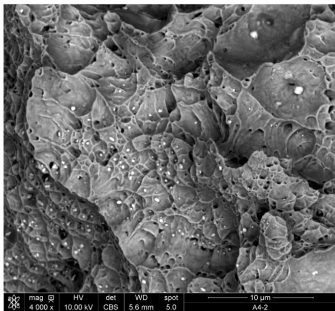
Fig. 4. SEM image of a fracture surface of a tensile specimen (austenitization performed at 1020 °C).
