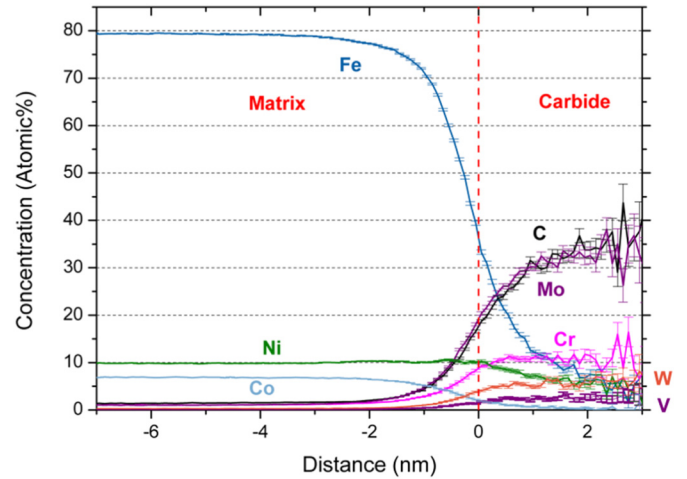
Fig. 14. Proximity histogram of the 98 interfaces precipitate/matrix.
