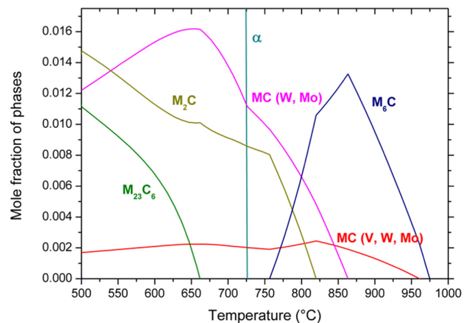
Fig. 2. Mole fraction of phase according to austenitizing temperature in M54® calculated with TCFE3 ThermoCalc® database (Ti-free).
