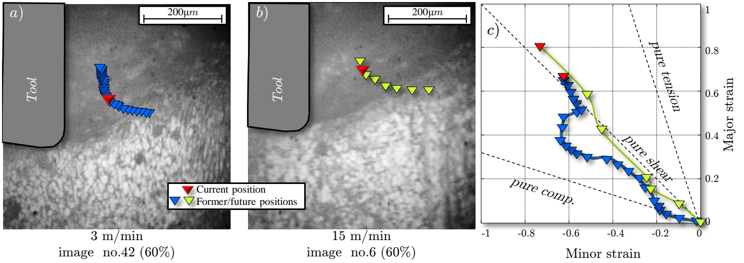
Figure 10: a) Trajectory of the considered point, up to material failure, for the test at 3 m \cdot min^{-1} . b) Trajectory of the considered point, up to material failure for the test at 15 m \cdot min^{-1} . c) Strain path up to failure for both considered points (cutting speed) in the strain principal plane.
