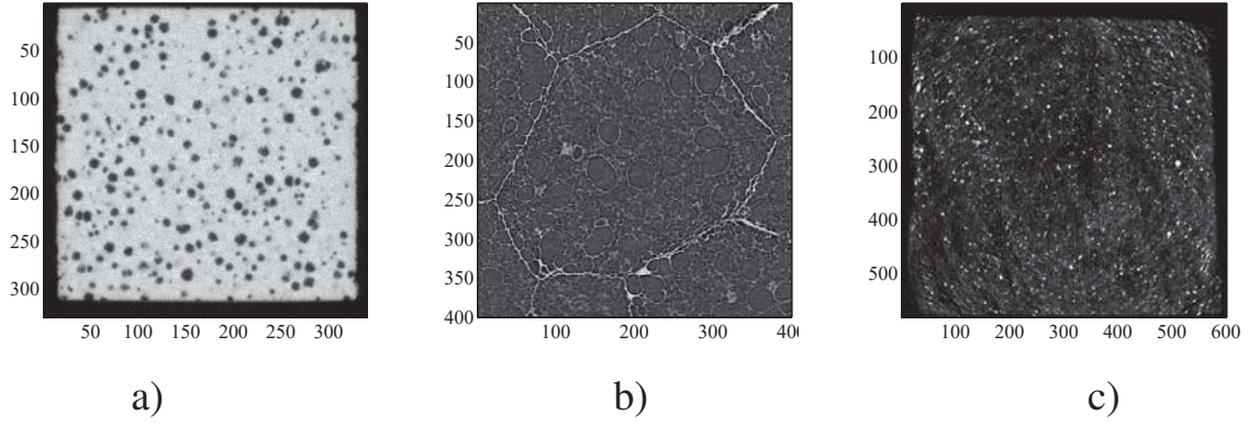
Figure 6.3. Examples of sections through 3D X-rays computed tomography images; a) Cast iron with spheroidal graphite modules; b) Polymeric foam; c) Stonewool
