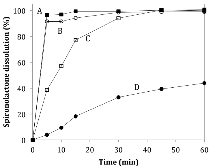
Figure 6. Dissolution of Spironolactone from HME formulations (A, B, C) in comparison with unprocessed microcrystalline Spironolactone (D). (A, B) CO 2 -foamed-extruded and ground, (C) CO 2 -foamed sample.
