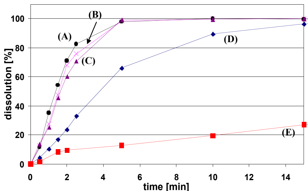
Figure 5. Dissolution of Carvedilol from HME formulations (A, B, C, D) in comparison to unprocessed crystalline Carvedilol (E). (A) CO 2 -foamed-extruded and ground, (B) extruded and ground, (C) extruded, (D) CO 2 -foamed sample.
