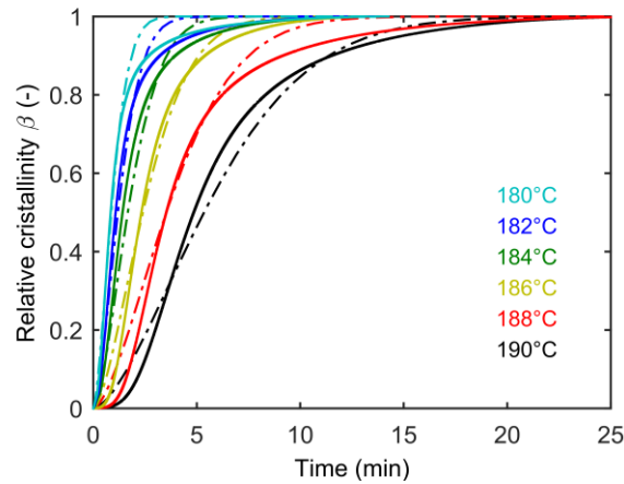
Figure 4: Crystallization modeling from molten state
