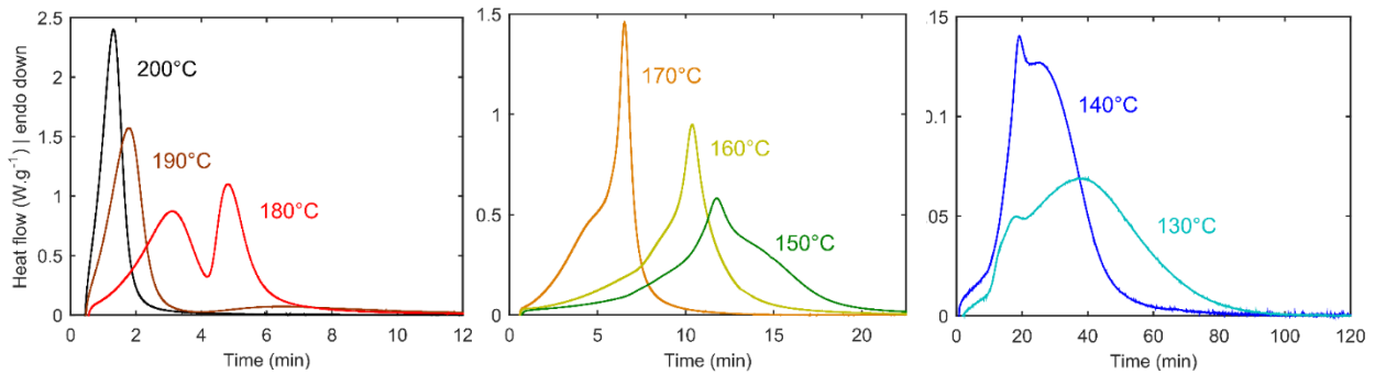
Figure 1: DSC curves of isothermal syntheses of PA6
