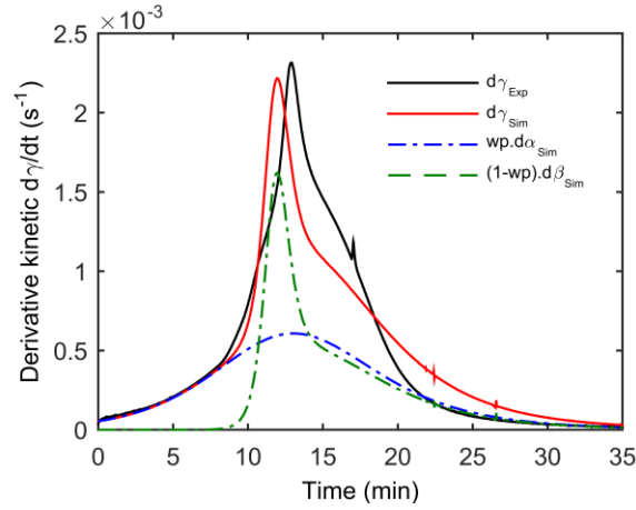
Figure 6: Modeling with equation 7 at 150°C
