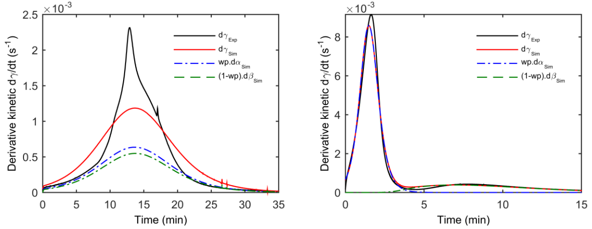
Figure 5: Modeling with equation 5 syntheses at (a) 150°C, (b) 190°C
