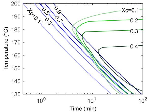
Figure 7: TTT diagram (blue: degree of conversion X_p , green: degree of crystallization X_c )
