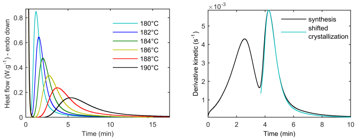
Figure 3: DSC scans of crystallization from molten state (a) isothermal steps, (b) synthesis superposition at 180^\circ\text{C}
