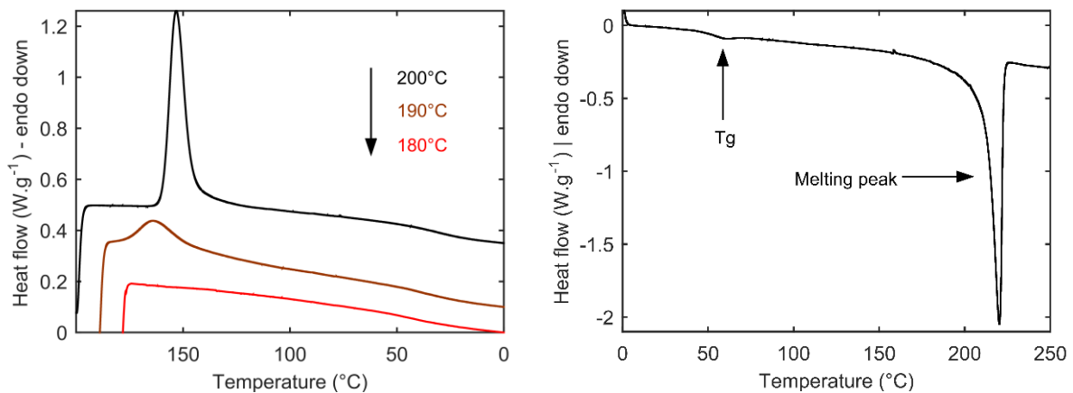
Figure 2: DSC scans of the cooling step (a), heating (b)
