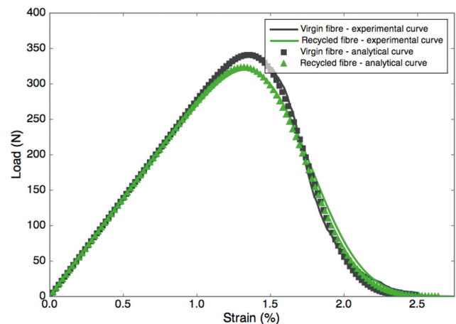
Fig. 4: Tests on tows. Experimental and analytical load-strain curves for virgin and recycled carbon fibre. The difference recorded at maximum load is due to the difference in the number of filaments in the tows
