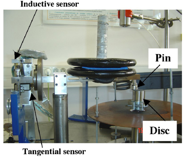
Fig. 1. General view of the pin-on-disc tribometer.
