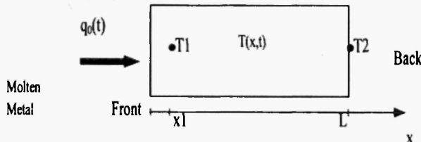
Fig. 1 : One dimensional heat conduction system (20).
