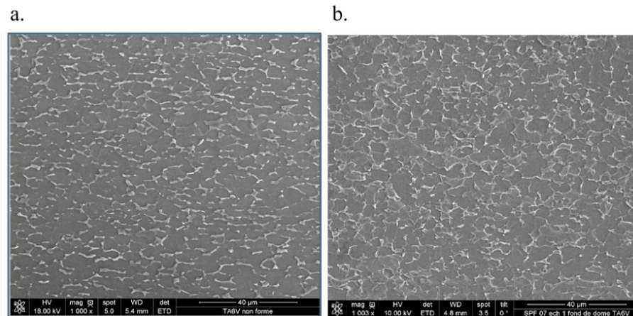
Figure 5: (a.) SEM image of the TA6V microstructure before forming shows the classical \alpha+\beta phases, (b.) SEM image of the TA6V microstructure after forming shows that the \alpha+\beta phases are conserved.
