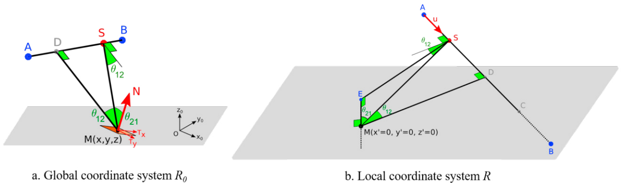
Figure 1: (a.) View factor from a point S in lamp [AB] to a point M on a non-plane sheet with a normal vector \vec{N} . (b) Lamp and sheet after changing the global coordinate system \mathcal{R}_0(O, \vec{x}_0, \vec{y}_0, \vec{z}_0) for the local coordinate system \mathcal{R}(M, \vec{T}_x, \vec{T}_y, \vec{N}) .
