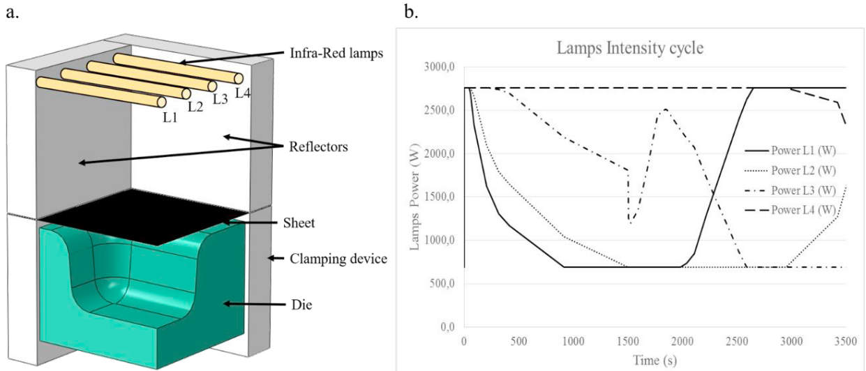
Figure 2: (a.) Schema of the laboratory device (only a quart of the device is represented) and (b.) lamps intensity cycle for the forming of a TA6V 500x500 mm 2 sheet obtained from the FEM simulation, coupling PID and new radiative flux model.
