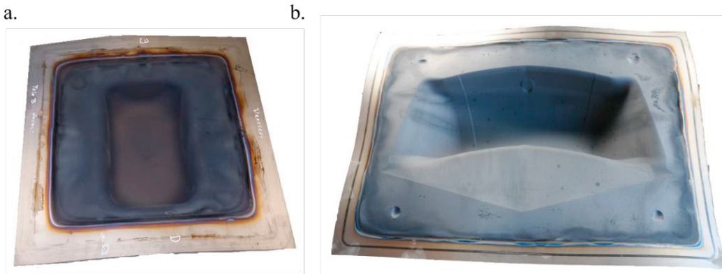
Figure 4: Examples of sheets of 500x500 mm 2 (a.) and 1500x1000 mm 2 (b.) formed by superplastic forming using Infra-Red lamps.
