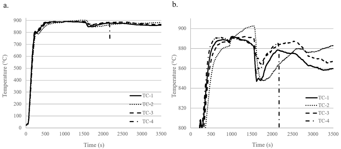
Figure 3: Sheet’s temperature measured by some thermocouples (TC) during a forming test: Global evolution (a.) and details of the temperature variations (b.).
