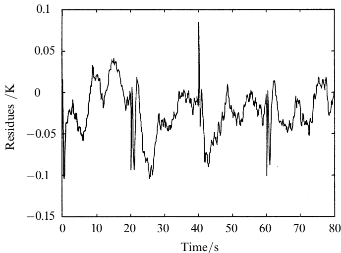
Figure 11. Computation of the residues ( \Delta t = 0.1 s).
