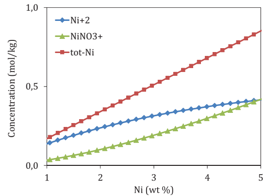
Fig. 4 Speciation of Ni using SIT model
