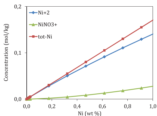
Fig. 3 Speciation of Ni using LLNL model
