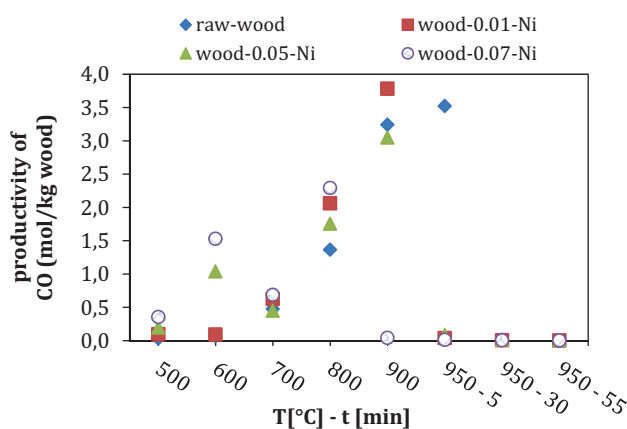
Fig. 12 Yield of CO production for all the samples
