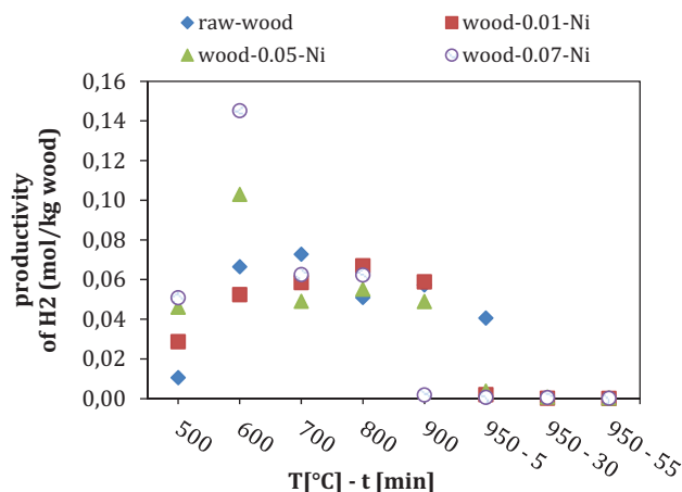
Fig. 13 Yield of H 2 production for all the samples
