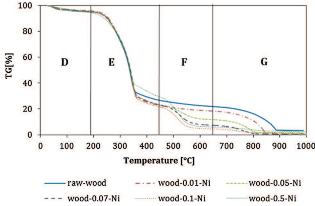
Fig. 9 TG profiles for wood samples impregnated during 24 h
