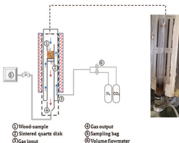
Fig. 1 Fixed bed Reactor
