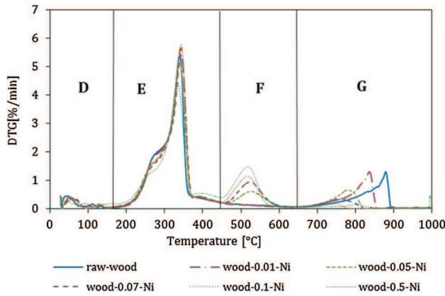
Fig. 10 DTG profiles of impregnated wood samples during 24 h
