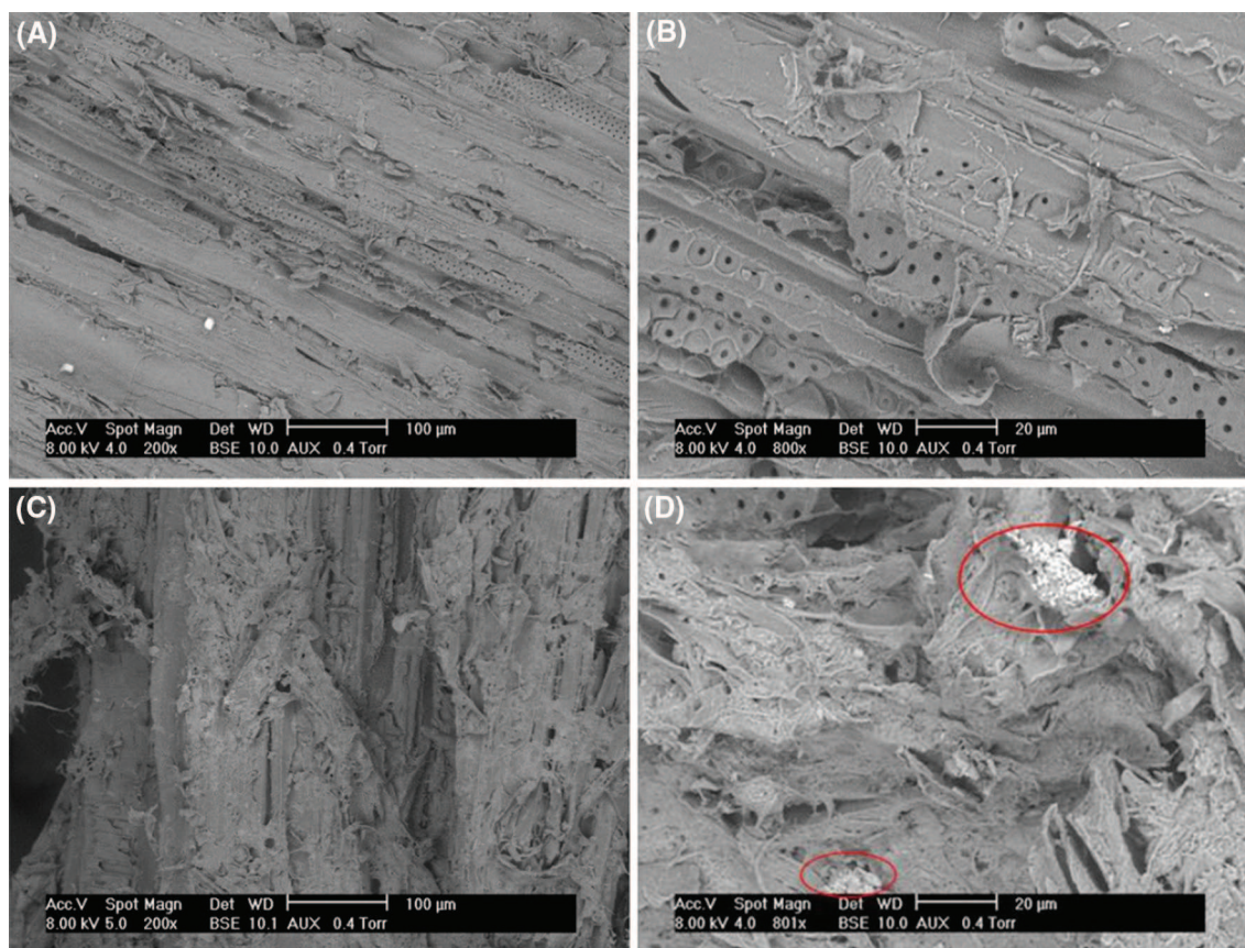
Fig. 5 SEM images of raw wood (A, B) and the wood-5-Ni sample (C, D)
