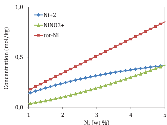
Fig. 4 Speciation of Ni using SIT model
