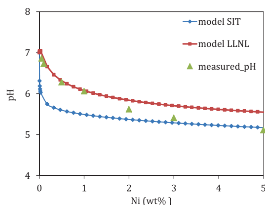
Fig. 2 Measured and calculated (according to two different models) pH variation of the nickel nitrate solutions at 25 °C
