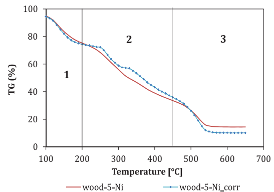
Fig. 8 TG profiles for wood-5-Ni with and without the decomposition of nickel nitrate
