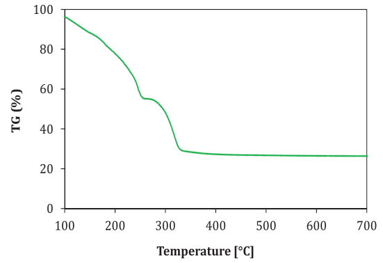
Fig. 7 Nickel nitrate degradation at 5 °C/min
