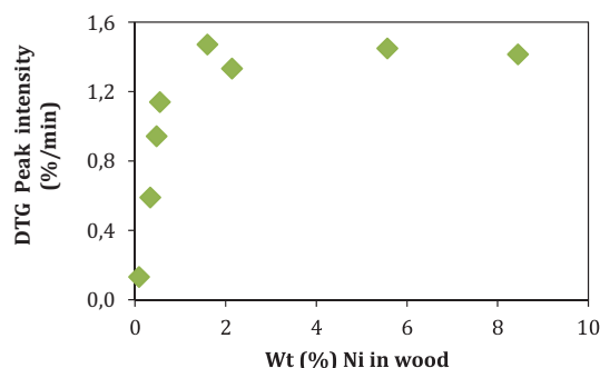
Fig. 11 Effect of the concentration of Ni on its catalytic effect at 520 °C
