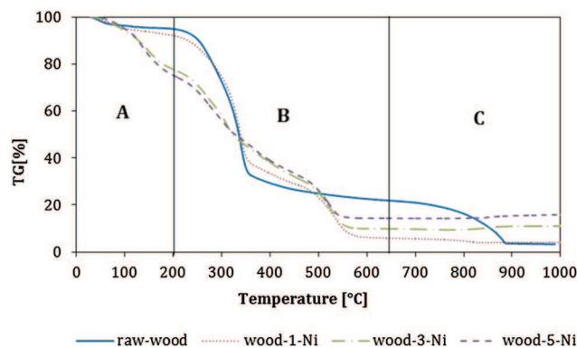
Fig. 6 TG profiles of wood samples impregnated during 3 days
